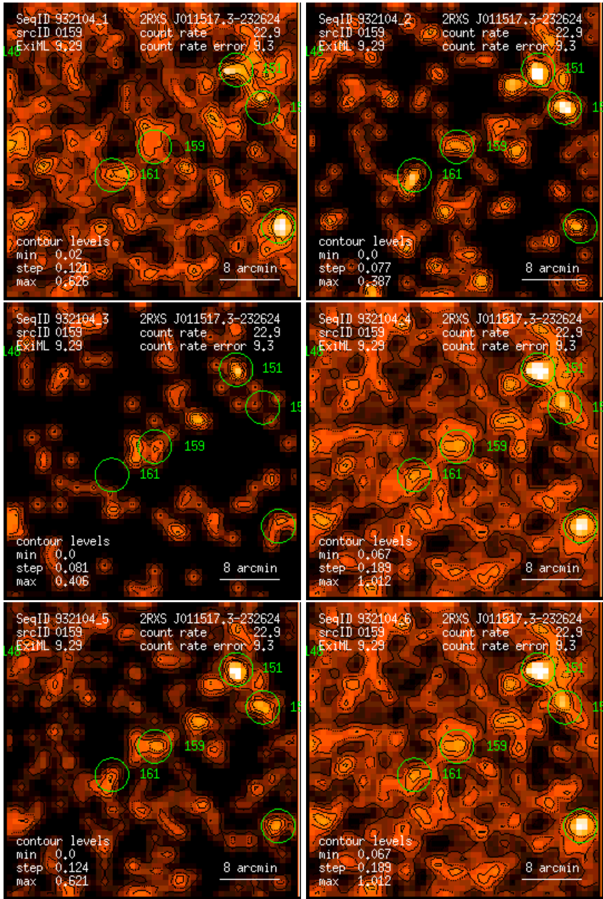
Figure 159: RASS 932104: detection 0159: band rate images, Gaussian filter: (1) PSPC channels 11 – 41, (2) 52 – 90, (3) 91 – 201, (4) 11 – 235, (5) 52 – 201, (6) 11 – 201. Broad band rates in counts/ks. Band rate contour levels in counts/ks/arcmin 2 .
