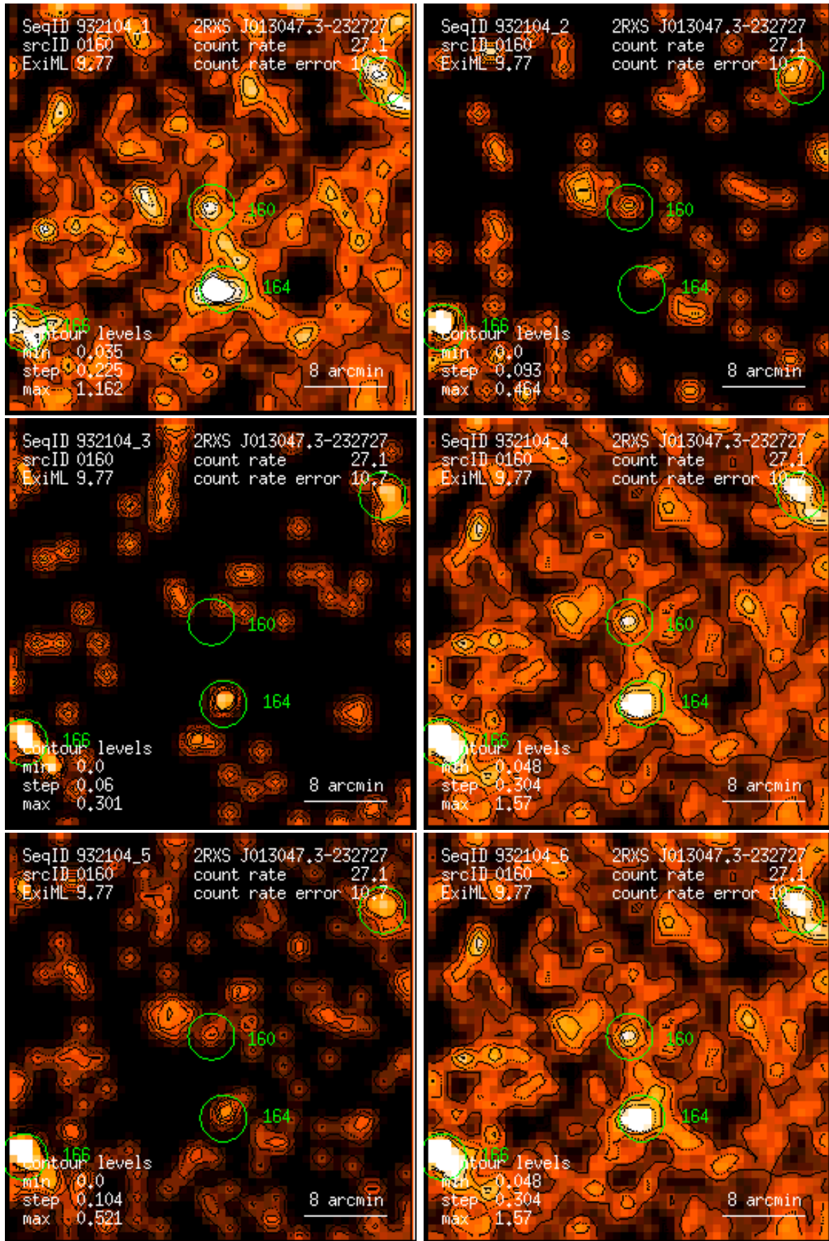
Figure 160: RASS 932104: detection 0160: band rate images, Gaussian filter: (1) PSPC channels 11 – 41, (2) 52 – 90, (3) 91 – 201, (4) 11 – 235, (5) 52 – 201, (6) 11 – 201. Broad band rates in counts/ks. Band rate contour levels in counts/ks/arcmin 2 .
