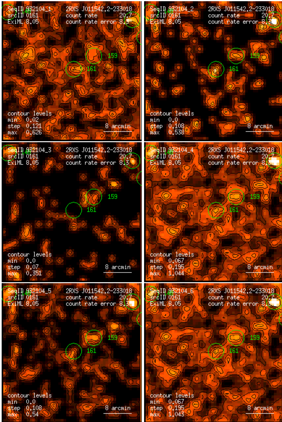
Figure 161: RASS 932104: detection 0161: band rate images, Gaussian filter: (1) PSPC channels 11 – 41, (2) 52 – 90, (3) 91 – 201, (4) 11 – 235, (5) 52 – 201, (6) 11 – 201. Broad band rates in counts/ks. Band rate contour levels in counts/ks/arcmin 2 .
