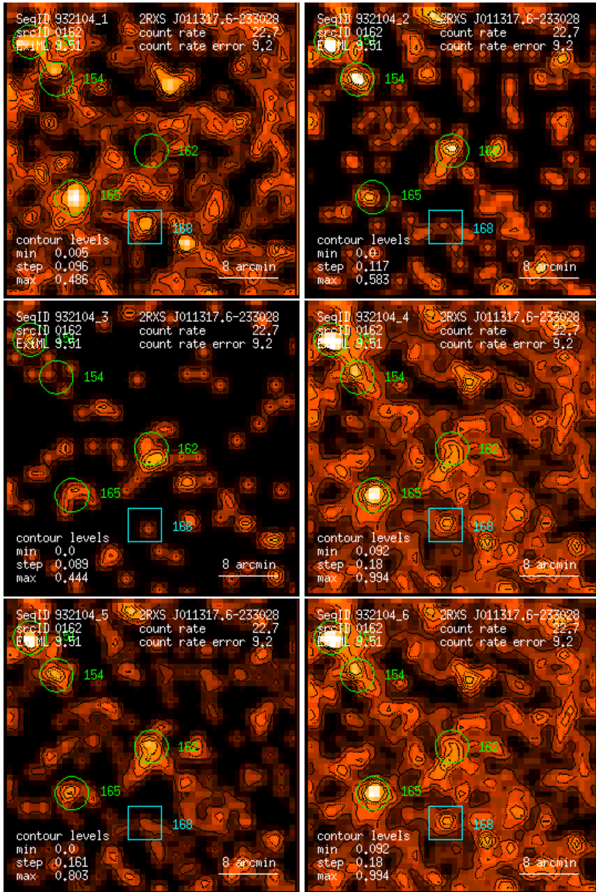
Figure 162: RASS 932104: detection 0162: band rate images, Gaussian filter: (1) PSPC channels 11 – 41, (2) 52 – 90, (3) 91 – 201, (4) 11 – 235, (5) 52 – 201, (6) 11 – 201. Broad band rates in counts/ks. Band rate contour levels in counts/ks/arcmin 2 .
