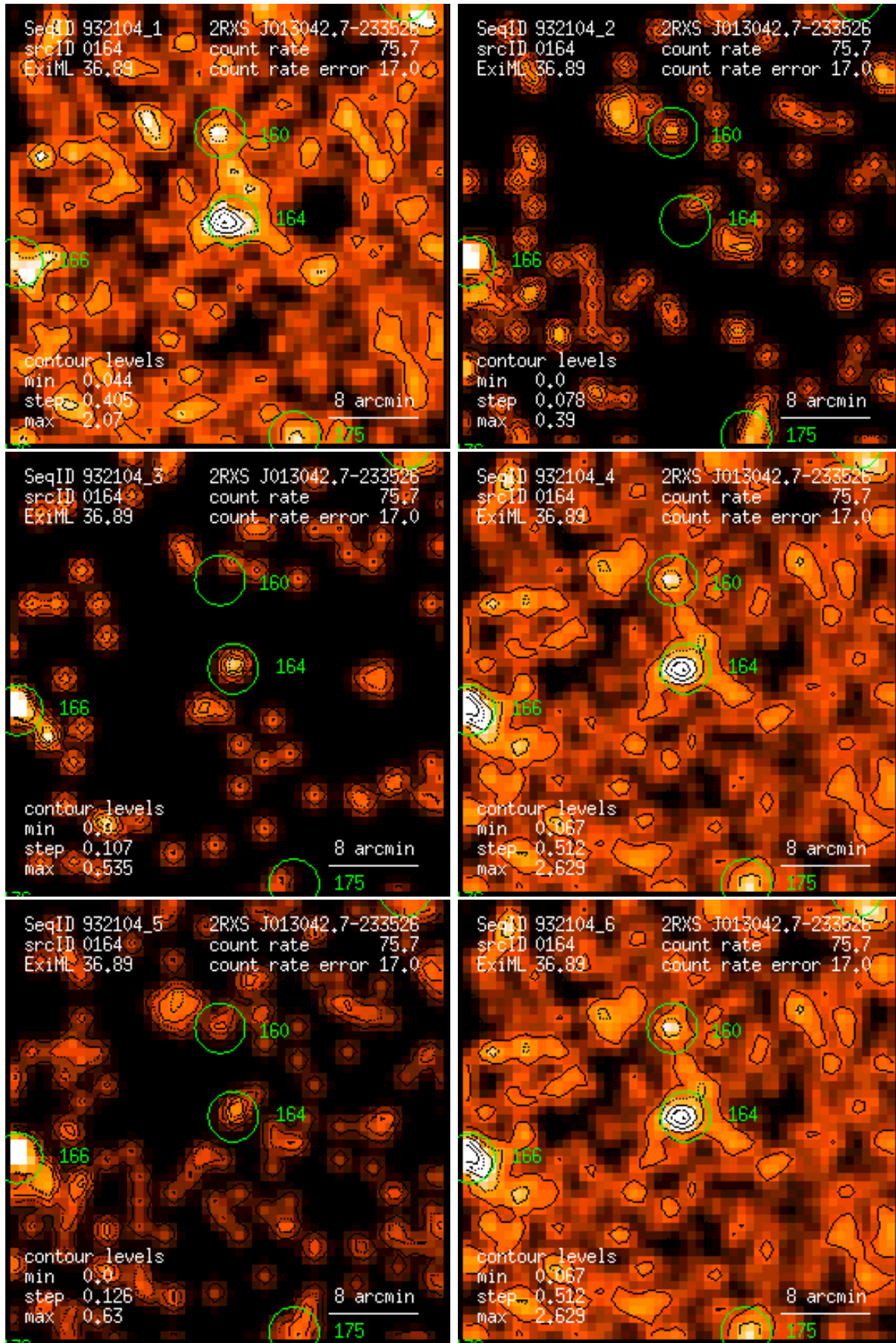
Figure 164: RASS 932104: detection 0164: band rate images, Gaussian filter: (1) PSPC channels 11 – 41, (2) 52 – 90, (3) 91 – 201, (4) 11 – 235, (5) 52 – 201, (6) 11 – 201. Broad band rates in counts/ks. Band rate contour levels in counts/ks/arcmin 2 .
