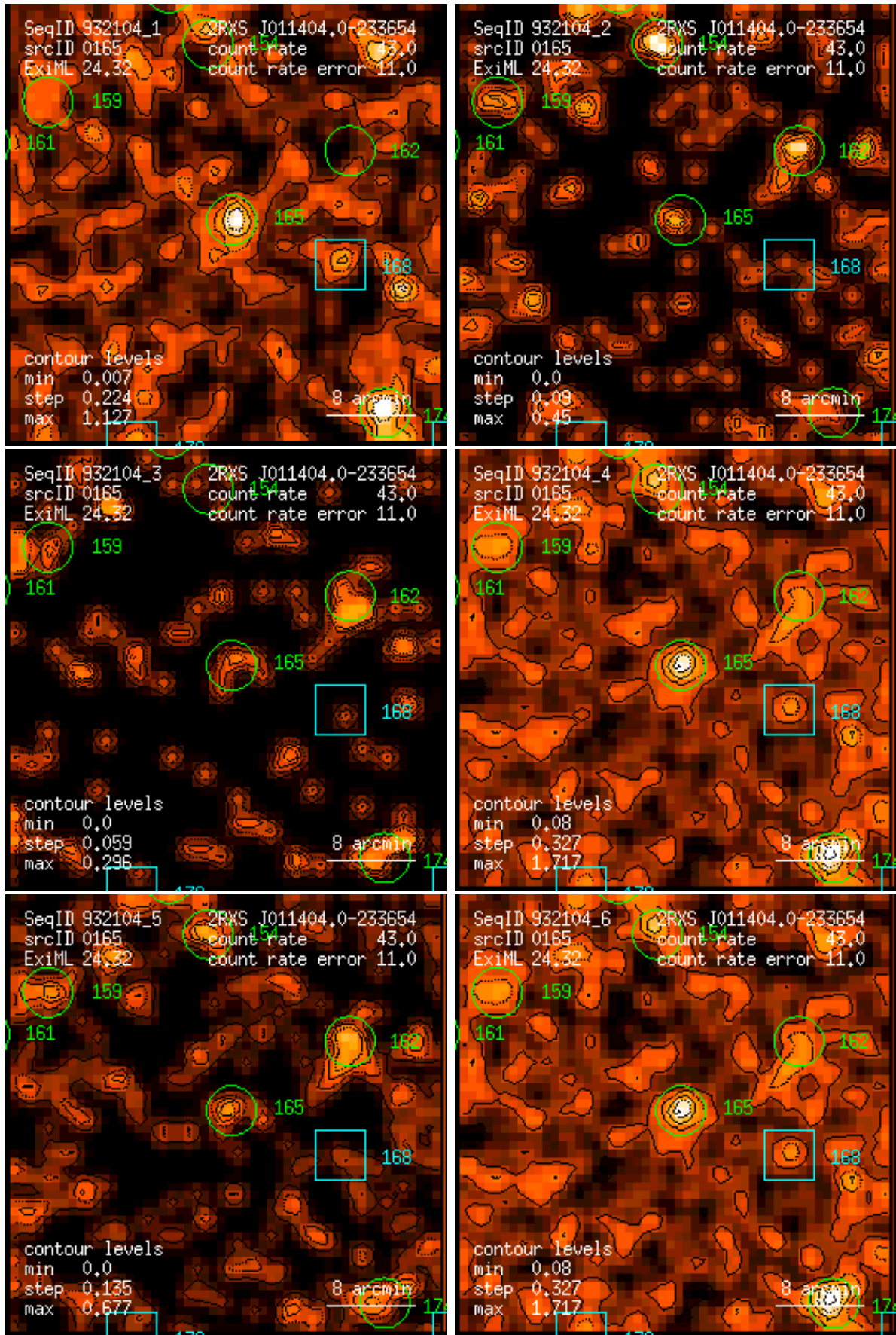
Figure 165: RASS 932104: detection 0165: band rate images, Gaussian filter: (1) PSPC channels 11 – 41, (2) 52 – 90, (3) 91 – 201, (4) 11 – 235, (5) 52 – 201, (6) 11 – 201. Broad band rates in counts/ks. Band rate contour levels in counts/ks/arcmin 2 .
