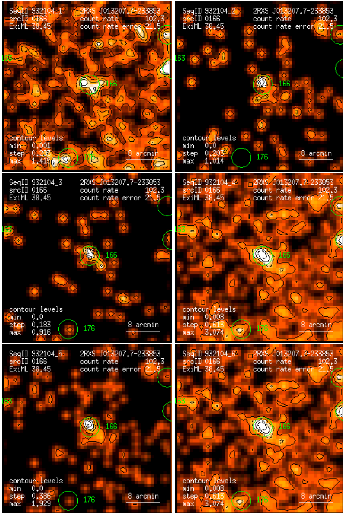
Figure 166: RASS 932104: detection 0166: band rate images, Gaussian filter: (1) PSPC channels 11 – 41, (2) 52 – 90, (3) 91 – 201, (4) 11 – 235, (5) 52 – 201, (6) 11 – 201. Broad band rates in counts/ks. Band rate contour levels in counts/ks/arcmin 2 .
