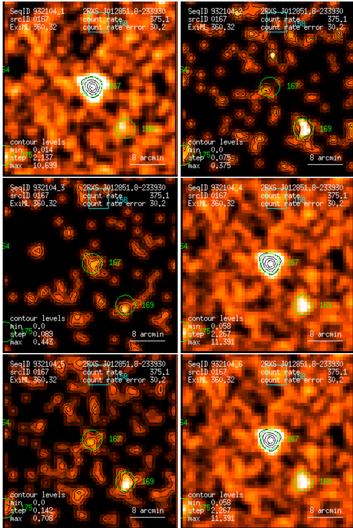
Figure 167: RASS 932104: detection 0167: band rate images, Gaussian filter: (1) PSPC channels 11 – 41, (2) 52 – 90, (3) 91 – 201, (4) 11 – 235, (5) 52 – 201, (6) 11 – 201. Broad band rates in counts/ks. Band rate contour levels in counts/ks/arcmin 2 .
