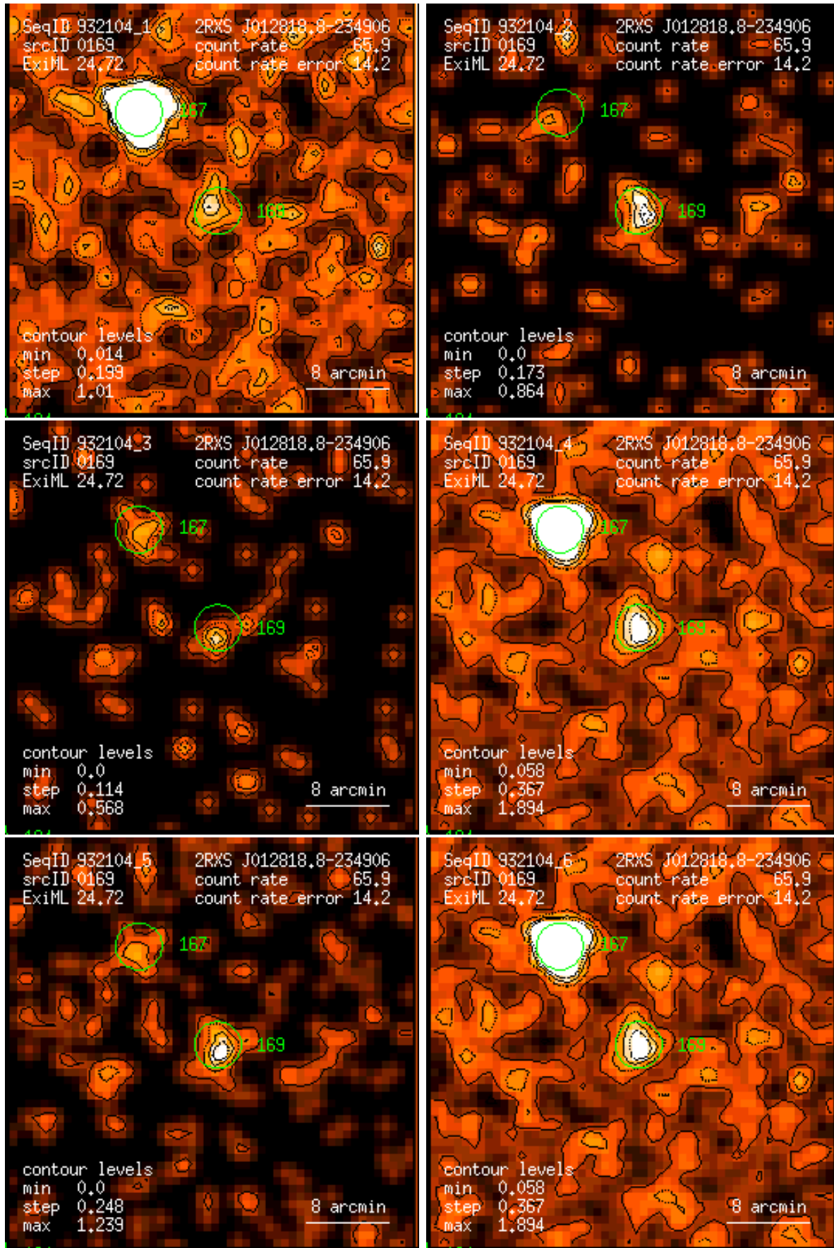
Figure 169: RASS 932104: detection 0169: band rate images, Gaussian filter: (1) PSPC channels 11 – 41, (2) 52 – 90, (3) 91 – 201, (4) 11 – 235, (5) 52 – 201, (6) 11 – 201. Broad band rates in counts/ks. Band rate contour levels in counts/ks/arcmin 2 .
