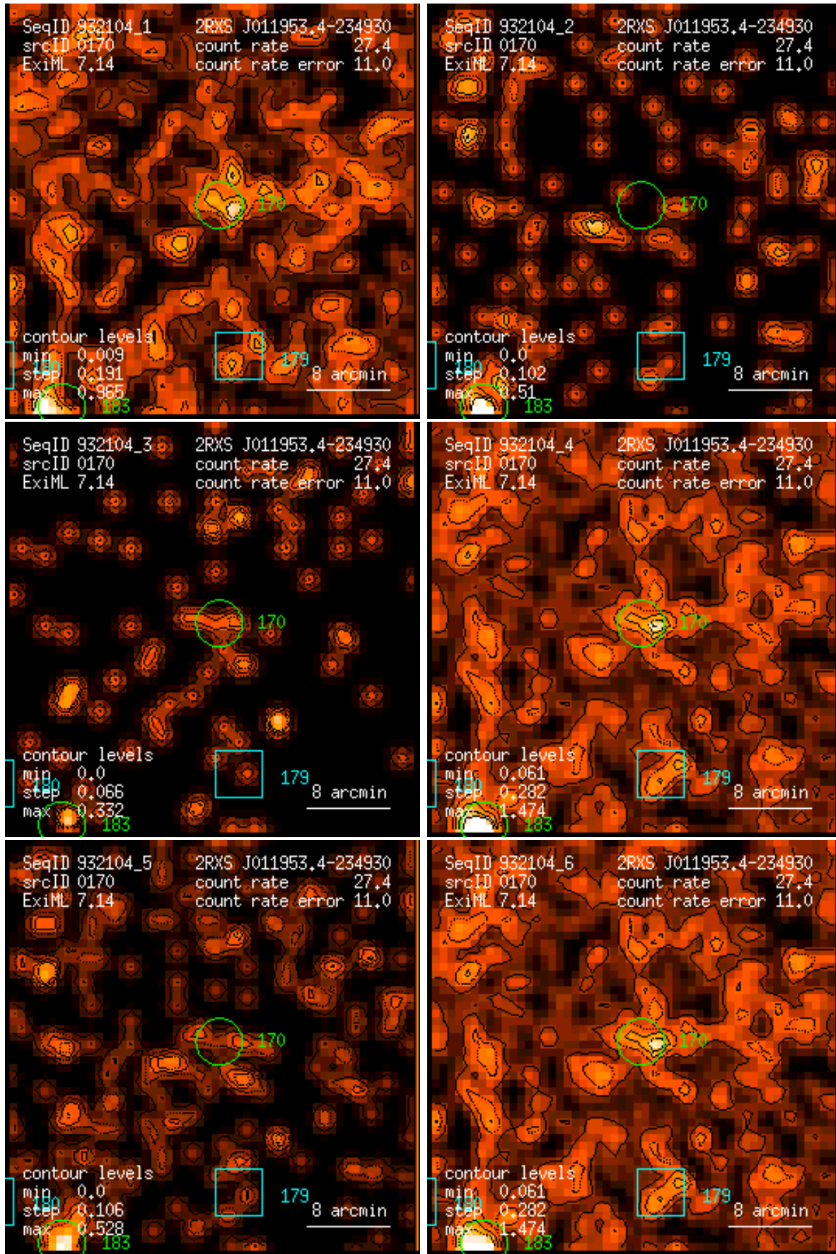
Figure 170: RASS 932104: detection 0170: band rate images, Gaussian filter: (1) PSPC channels 11 – 41, (2) 52 – 90, (3) 91 – 201, (4) 11 – 235, (5) 52 – 201, (6) 11 – 201. Broad band rates in counts/ks. Band rate contour levels in counts/ks/arcmin 2 .
