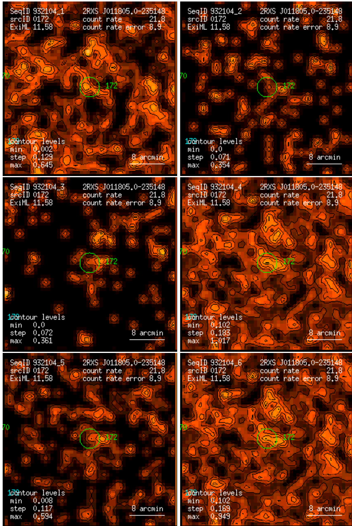
Figure 172: RASS 932104: detection 0172: band rate images, Gaussian filter: (1) PSPC channels 11 – 41, (2) 52 – 90, (3) 91 – 201, (4) 11 – 235, (5) 52 – 201, (6) 11 – 201. Broad band rates in counts/ks. Band rate contour levels in counts/ks/arcmin 2 .
