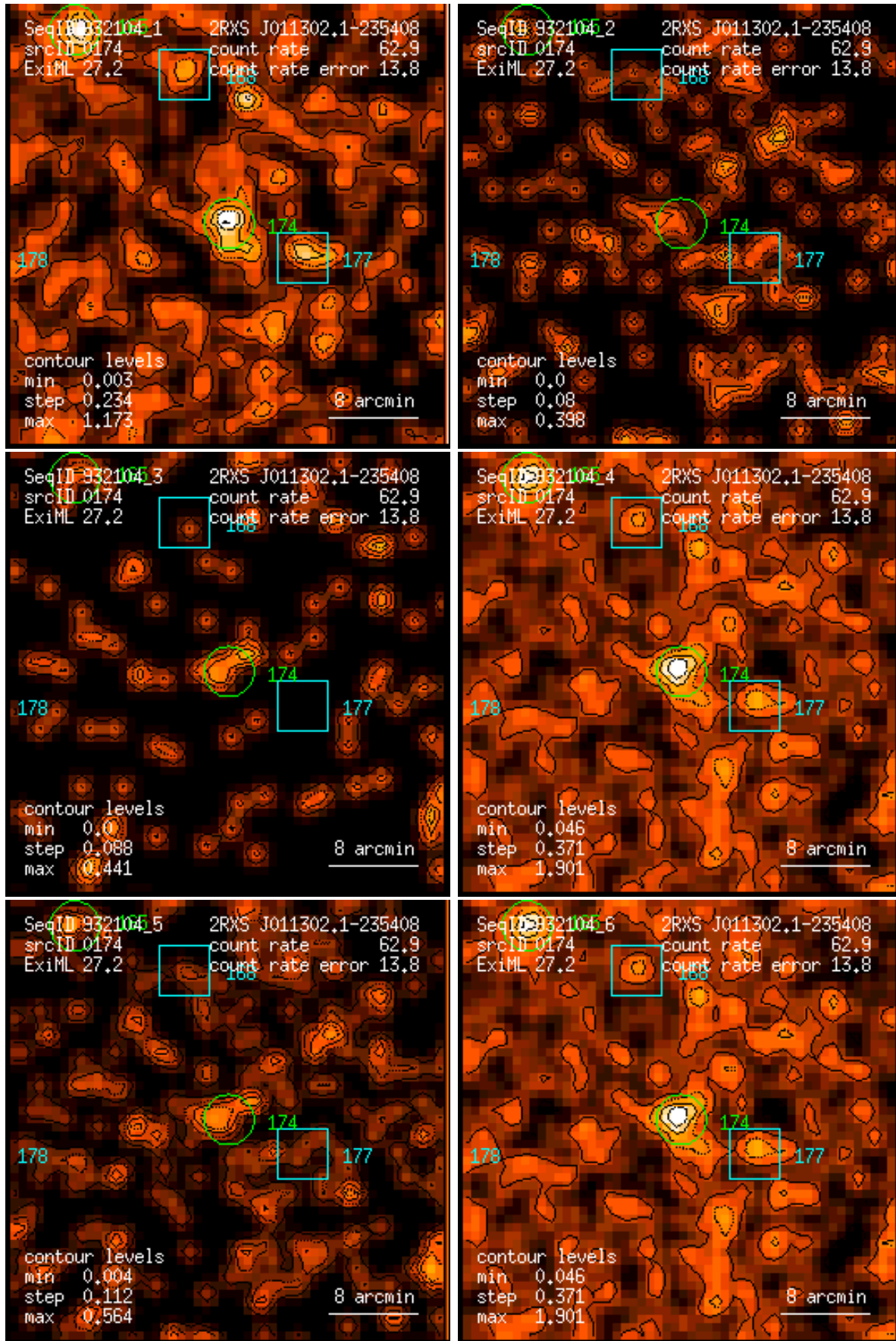
Figure 174: RASS 932104: detection 0174: band rate images, Gaussian filter: (1) PSPC channels 11 – 41, (2) 52 – 90, (3) 91 – 201, (4) 11 – 235, (5) 52 – 201, (6) 11 – 201. Broad band rates in counts/ks. Band rate contour levels in counts/ks/arcmin 2 .
