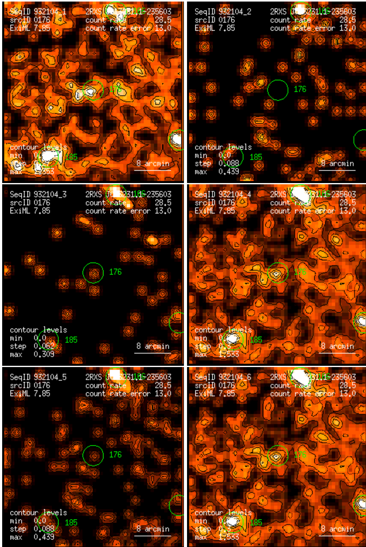
Figure 176: RASS 932104: detection 0176: band rate images, Gaussian filter: (1) PSPC channels 11 – 41, (2) 52 – 90, (3) 91 – 201, (4) 11 – 235, (5) 52 – 201, (6) 11 – 201. Broad band rates in counts/ks. Band rate contour levels in counts/ks/arcmin 2 .
