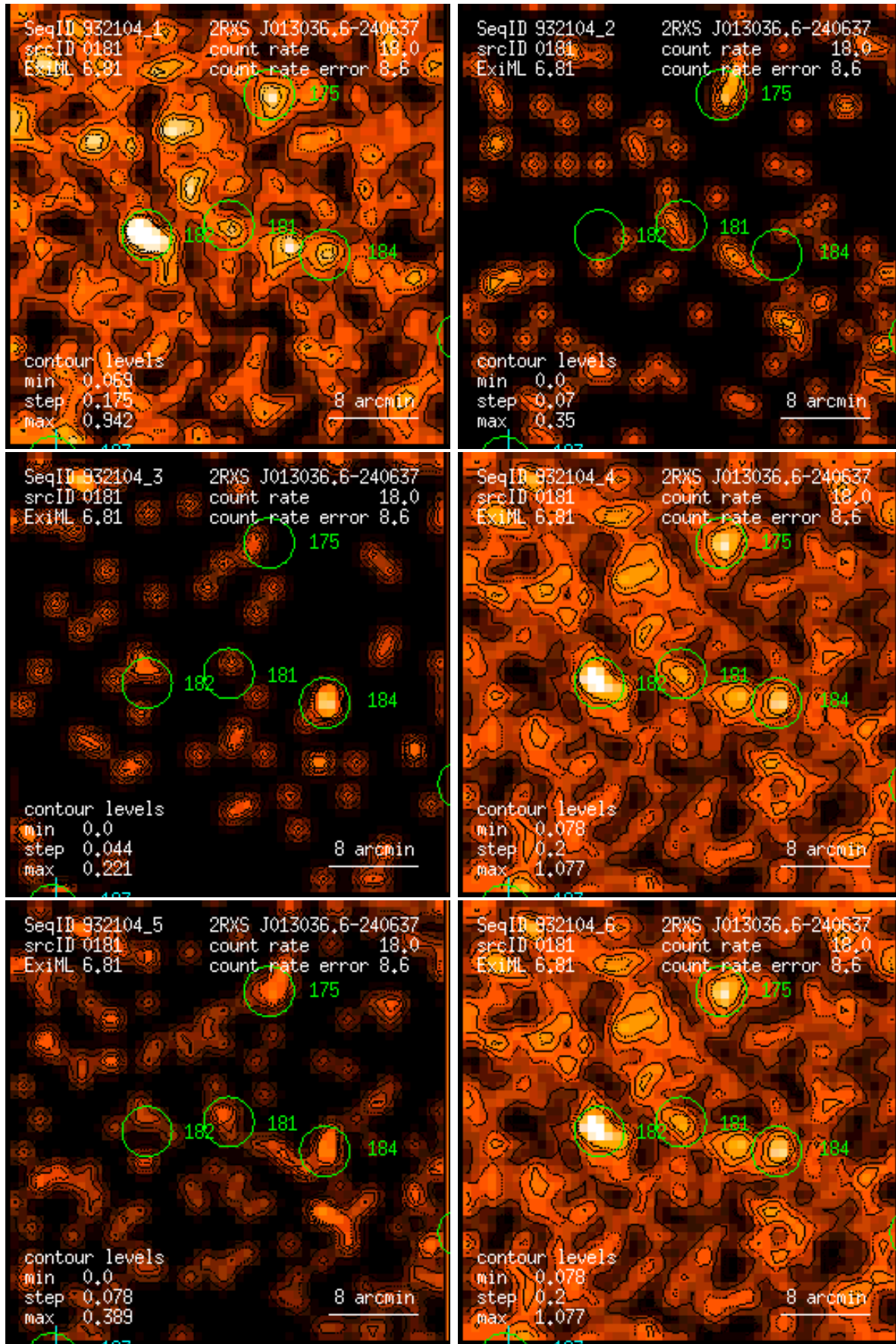
Figure 181: RASS 932104: detection 0181: band rate images, Gaussian filter: (1) PSPC channels 11 – 41, (2) 52 – 90, (3) 91 – 201, (4) 11 – 235, (5) 52 – 201, (6) 11 – 201. Broad band rates in counts/ks. Band rate contour levels in counts/ks/arcmin 2 .
