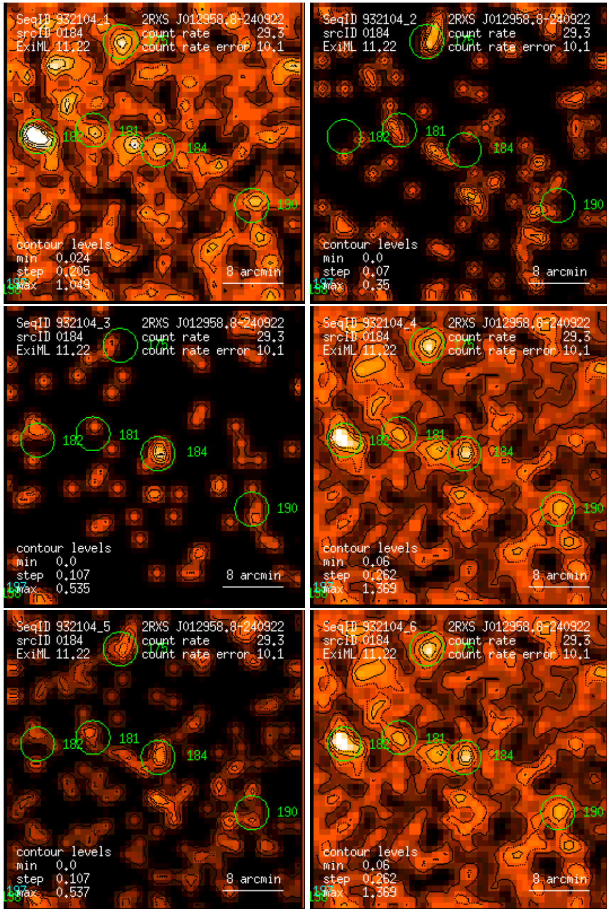
Figure 184: RASS 932104: detection 0184: band rate images, Gaussian filter: (1) PSPC channels 11 – 41, (2) 52 – 90, (3) 91 – 201, (4) 11 – 235, (5) 52 – 201, (6) 11 – 201. Broad band rates in counts/ks. Band rate contour levels in counts/ks/arcmin 2 .
