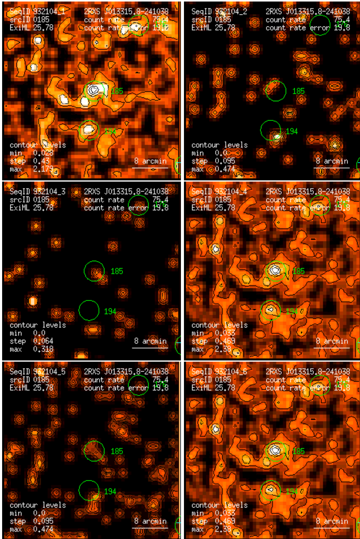
Figure 185: RASS 932104: detection 0185: band rate images, Gaussian filter: (1) PSPC channels 11 – 41, (2) 52 – 90, (3) 91 – 201, (4) 11 – 235, (5) 52 – 201, (6) 11 – 201. Broad band rates in counts/ks. Band rate contour levels in counts/ks/arcmin 2 .
