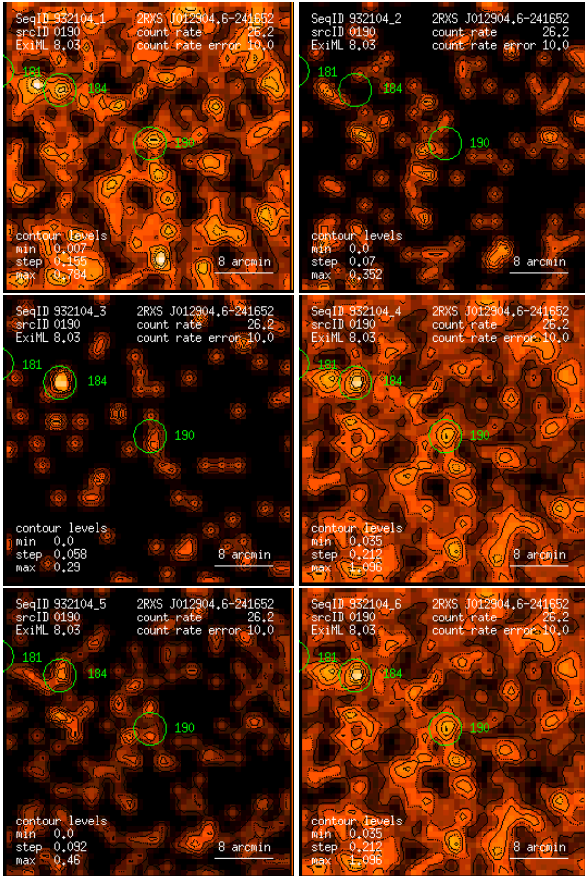
Figure 190: RASS 932104: detection 0190: band rate images, Gaussian filter: (1) PSPC channels 11 – 41, (2) 52 – 90, (3) 91 – 201, (4) 11 – 235, (5) 52 – 201, (6) 11 – 201. Broad band rates in counts/ks. Band rate contour levels in counts/ks/arcmin 2 .
