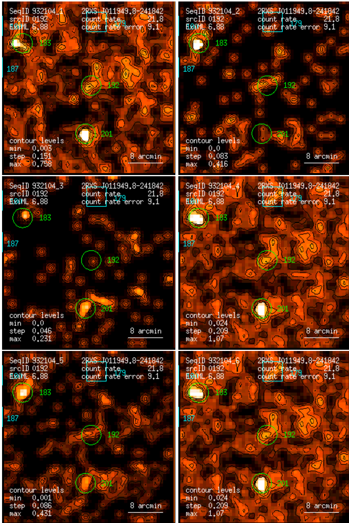
Figure 192: RASS 932104: detection 0192: band rate images, Gaussian filter: (1) PSPC channels 11 – 41, (2) 52 – 90, (3) 91 – 201, (4) 11 – 235, (5) 52 – 201, (6) 11 – 201. Broad band rates in counts/ks. Band rate contour levels in counts/ks/arcmin 2 .
