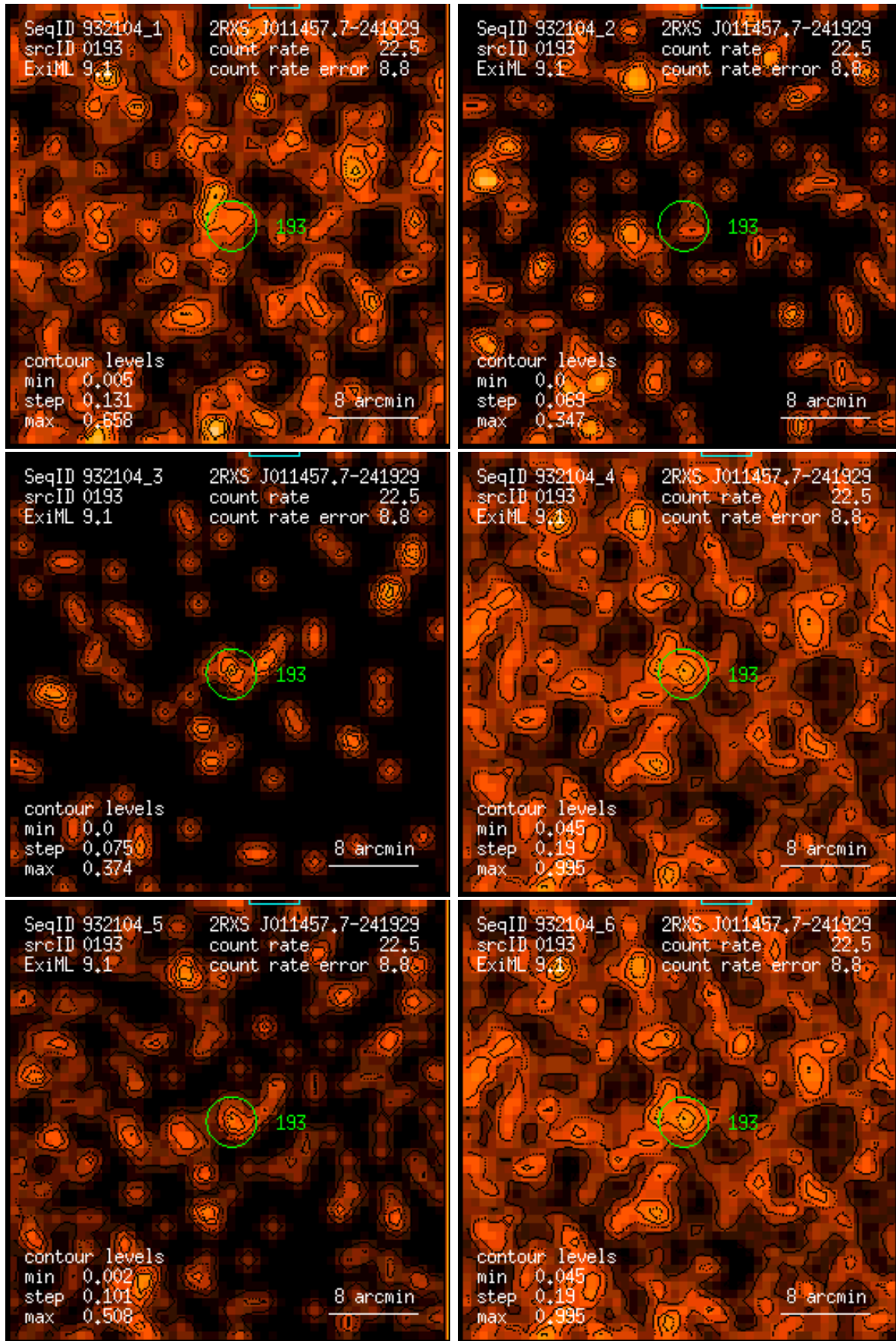
Figure 193: RASS 932104: detection 0193: band rate images, Gaussian filter: (1) PSPC channels 11 – 41, (2) 52 – 90, (3) 91 – 201, (4) 11 – 235, (5) 52 – 201, (6) 11 – 201. Broad band rates in counts/ks. Band rate contour levels in counts/ks/arcmin 2 .
