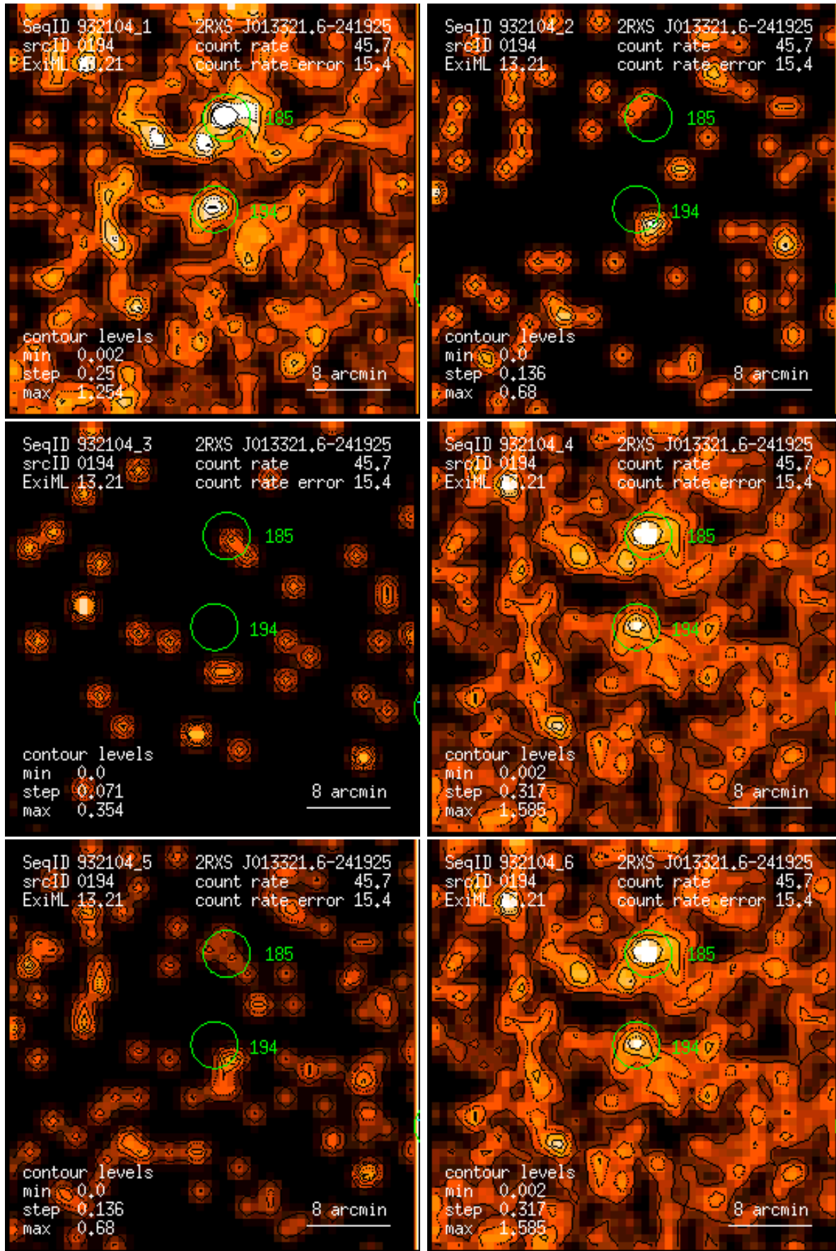
Figure 194: RASS 932104: detection 0194: band rate images, Gaussian filter: (1) PSPC channels 11 – 41, (2) 52 – 90, (3) 91 – 201, (4) 11 – 235, (5) 52 – 201, (6) 11 – 201. Broad band rates in counts/ks. Band rate contour levels in counts/ks/arcmin 2 .
