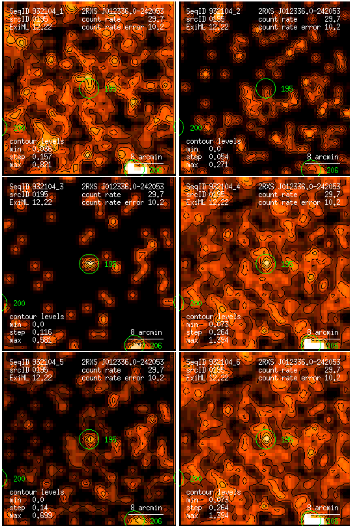
Figure 195: RASS 932104: detection 0195: band rate images, Gaussian filter: (1) PSPC channels 11 – 41, (2) 52 – 90, (3) 91 – 201, (4) 11 – 235, (5) 52 – 201, (6) 11 – 201. Broad band rates in counts/ks. Band rate contour levels in counts/ks/arcmin 2 .
