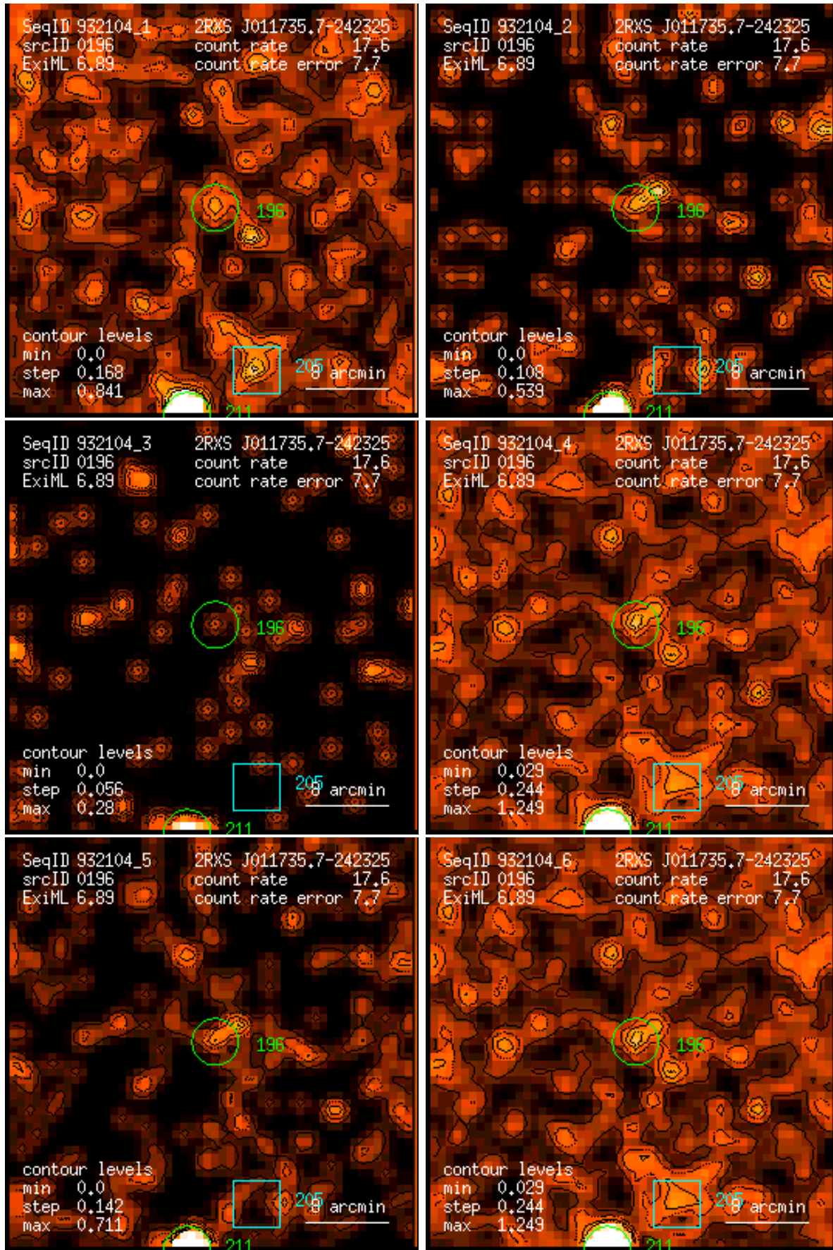
Figure 196: RASS 932104: detection 0196: band rate images, Gaussian filter: (1) PSPC channels 11 – 41, (2) 52 – 90, (3) 91 – 201, (4) 11 – 235, (5) 52 – 201, (6) 11 – 201. Broad band rates in counts/ks. Band rate contour levels in counts/ks/arcmin 2 .
