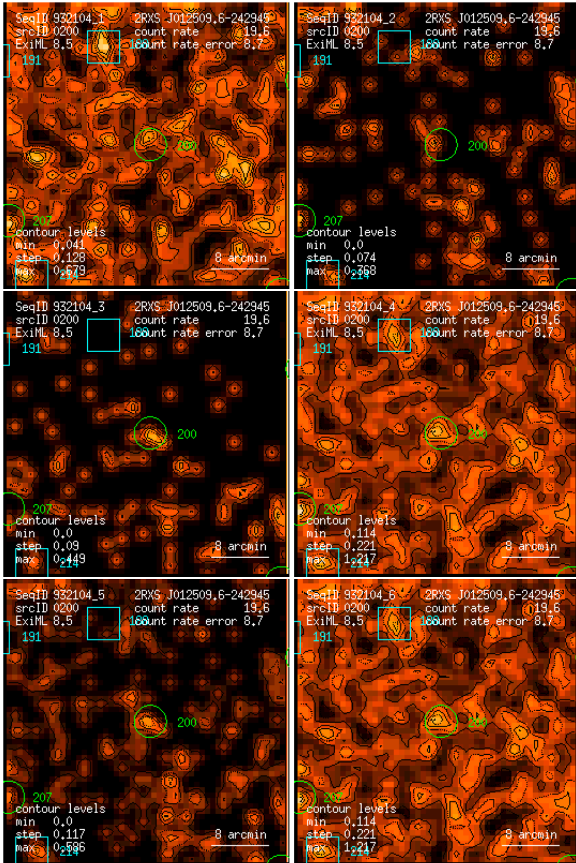
Figure 200: RASS 932104: detection 0200: band rate images, Gaussian filter: (1) PSPC channels 11 – 41, (2) 52 – 90, (3) 91 – 201, (4) 11 – 235, (5) 52 – 201, (6) 11 – 201. Broad band rates in counts/ks. Band rate contour levels in counts/ks/arcmin 2 .
