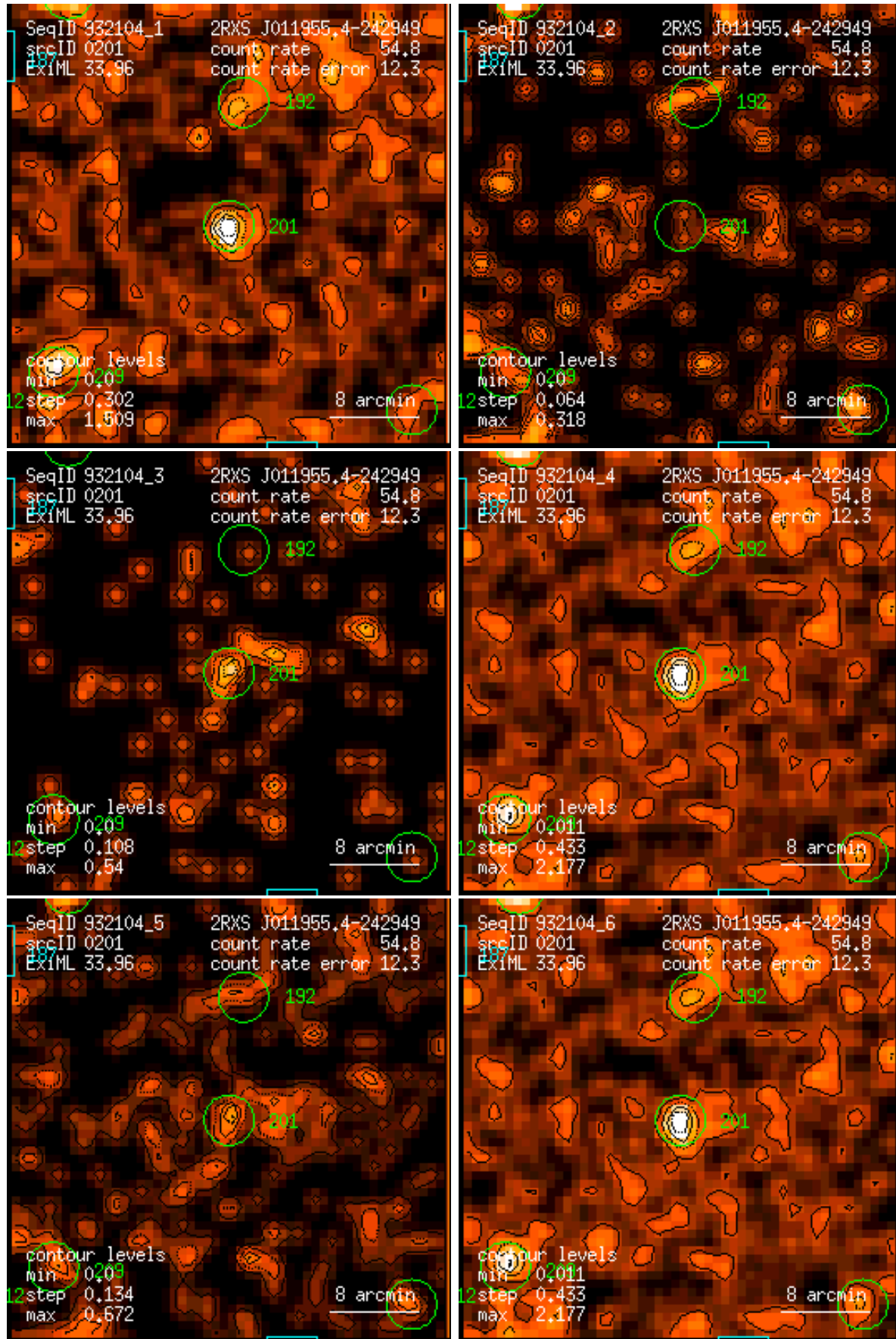
Figure 201: RASS 932104: detection 0201: band rate images, Gaussian filter: (1) PSPC channels 11 – 41, (2) 52 – 90, (3) 91 – 201, (4) 11 – 235, (5) 52 – 201, (6) 11 – 201. Broad band rates in counts/ks. Band rate contour levels in counts/ks/arcmin 2 .
