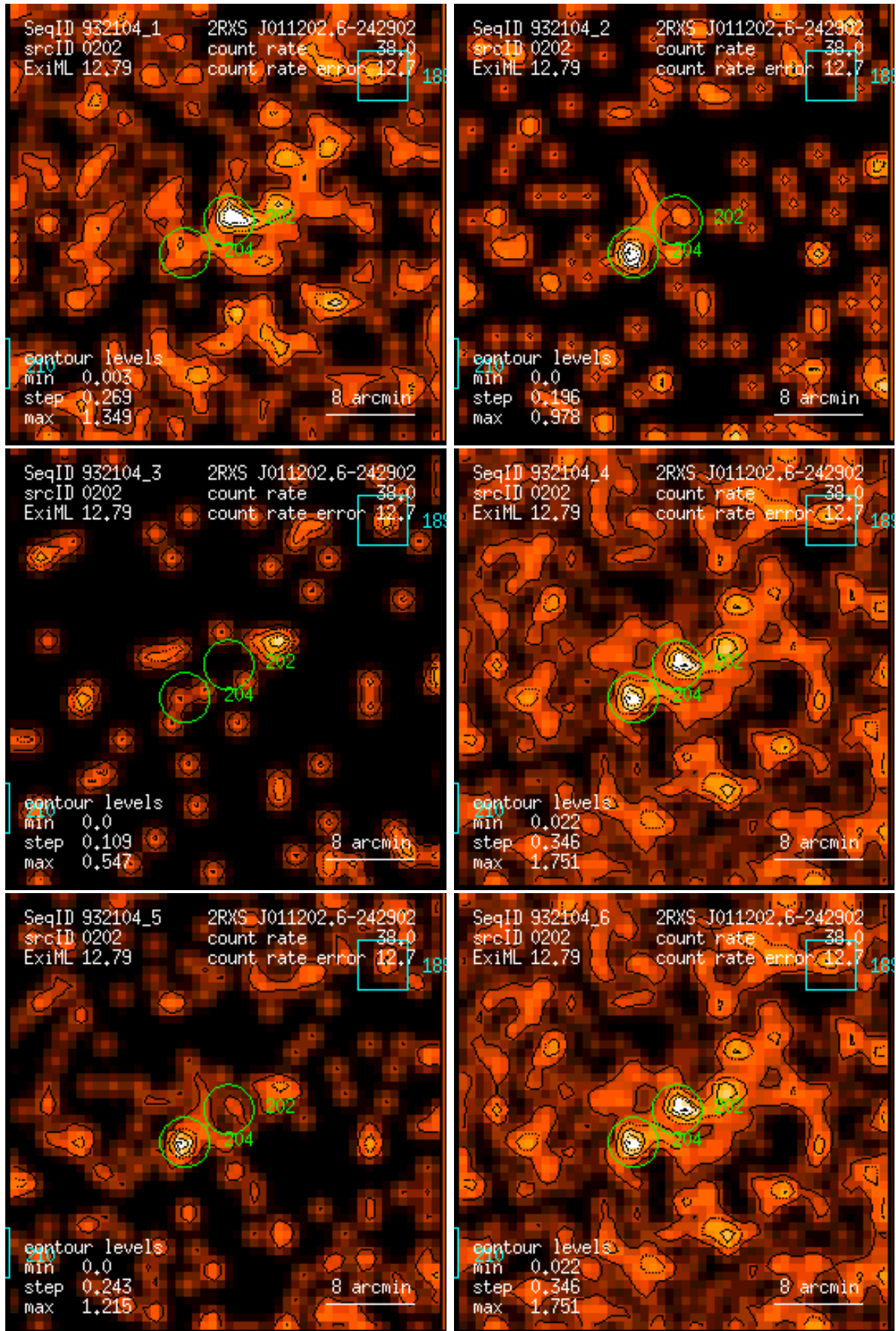
Figure 202: RASS 932104: detection 0202: band rate images, Gaussian filter: (1) PSPC channels 11 – 41, (2) 52 – 90, (3) 91 – 201, (4) 11 – 235, (5) 52 – 201, (6) 11 – 201. Broad band rates in counts/ks. Band rate contour levels in counts/ks/arcmin 2 .
