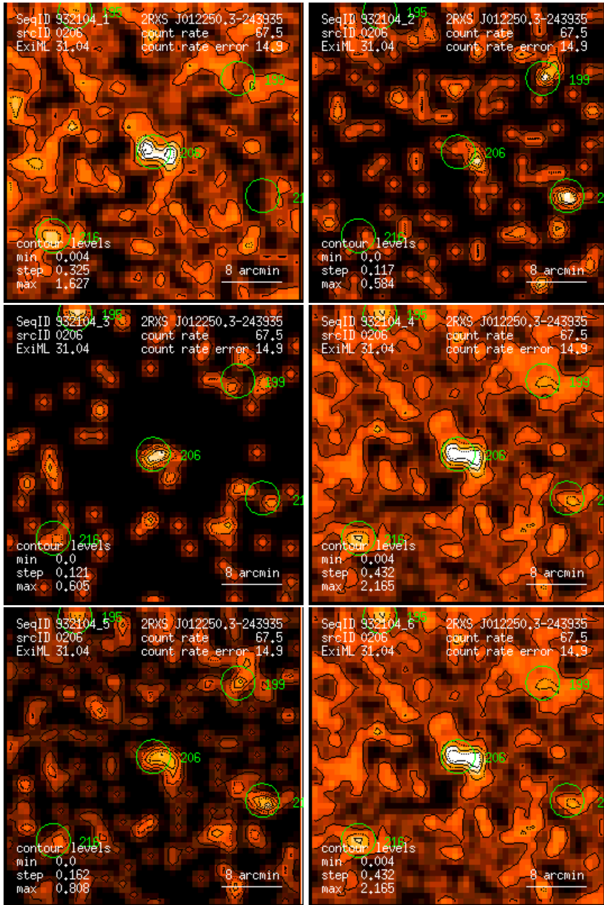
Figure 206: RASS 932104: detection 0206: band rate images, Gaussian filter: (1) PSPC channels 11 – 41, (2) 52 – 90, (3) 91 – 201, (4) 11 – 235, (5) 52 – 201, (6) 11 – 201. Broad band rates in counts/ks. Band rate contour levels in counts/ks/arcmin 2 .
