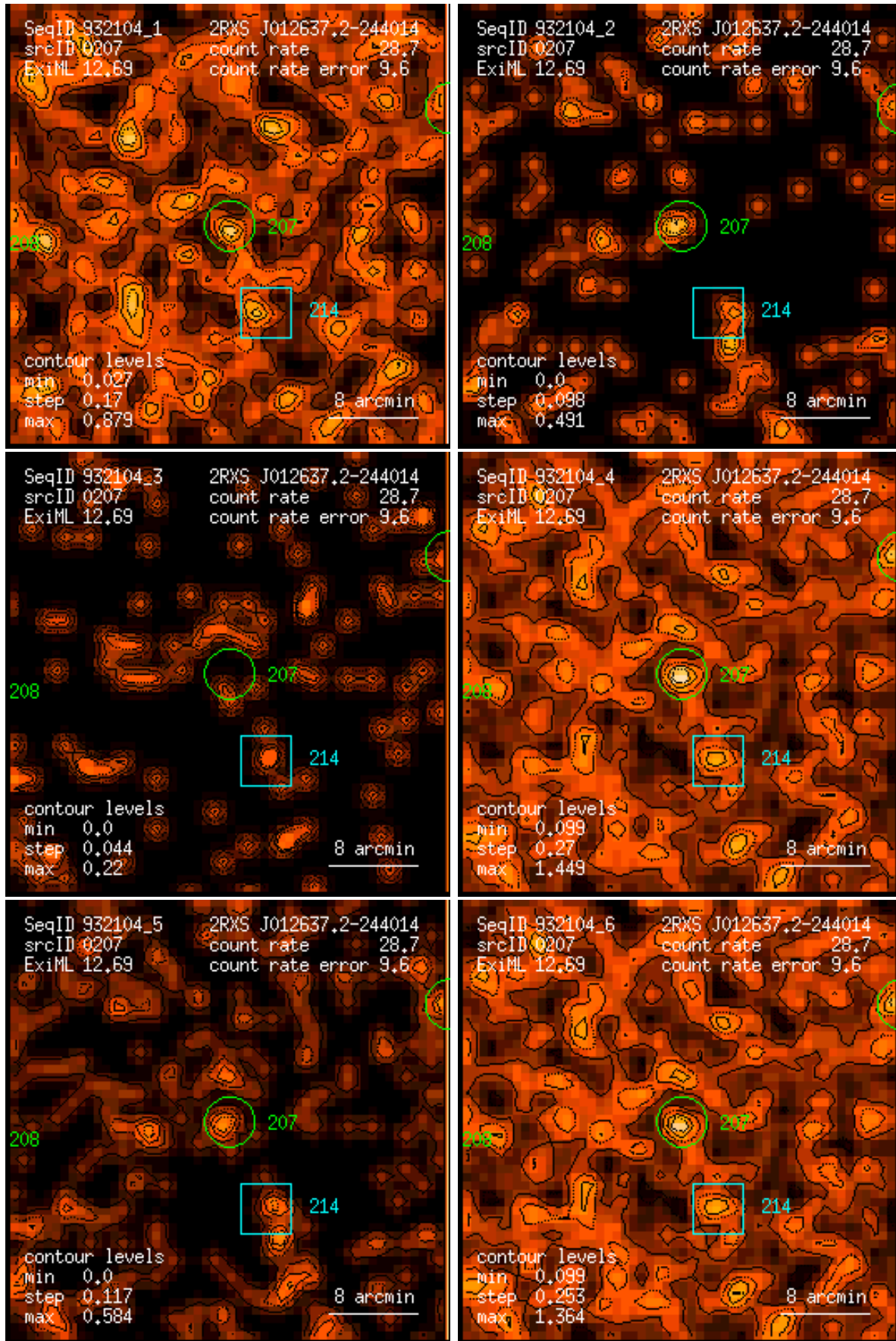
Figure 207: RASS 932104: detection 0207: band rate images, Gaussian filter: (1) PSPC channels 11 – 41, (2) 52 – 90, (3) 91 – 201, (4) 11 – 235, (5) 52 – 201, (6) 11 – 201. Broad band rates in counts/ks. Band rate contour levels in counts/ks/arcmin 2 .
