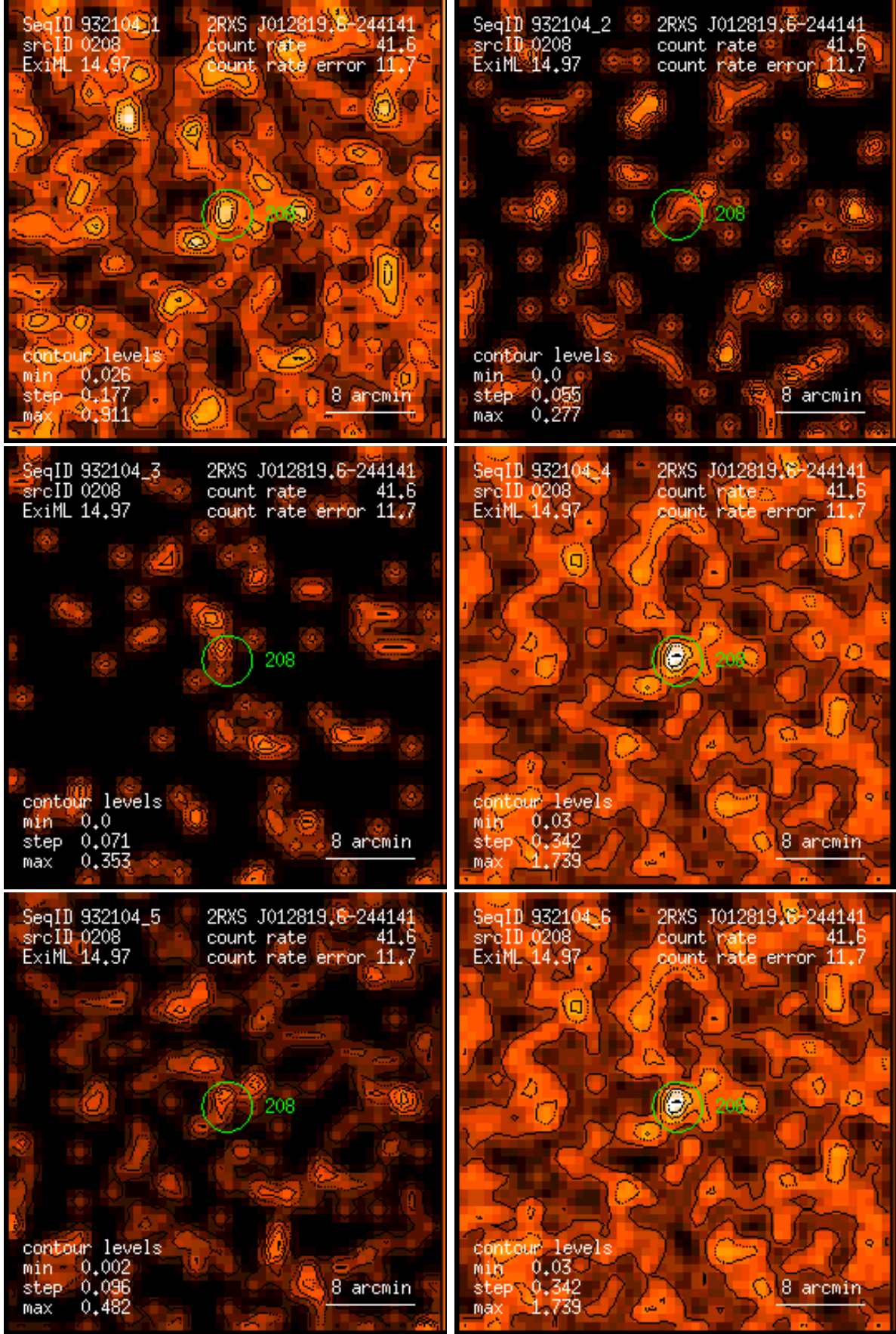
Figure 208: RASS 932104: detection 0208: band rate images, Gaussian filter: (1) PSPC channels 11 – 41, (2) 52 – 90, (3) 91 – 201, (4) 11 – 235, (5) 52 – 201, (6) 11 – 201. Broad band rates in counts/ks. Band rate contour levels in counts/ks/arcmin 2 .
