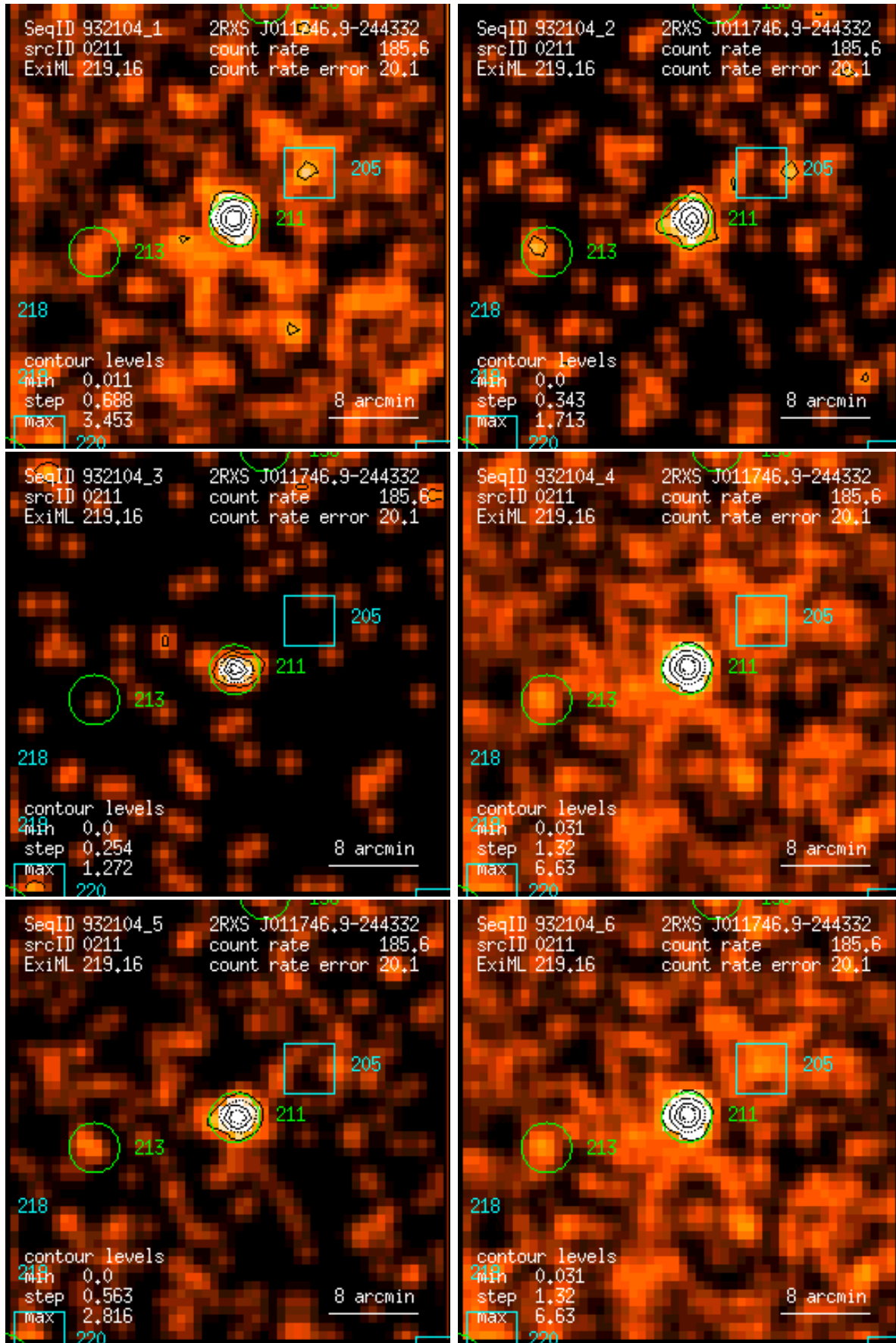
Figure 211: RASS 932104: detection 0211: band rate images, Gaussian filter: (1) PSPC channels 11 – 41, (2) 52 – 90, (3) 91 – 201, (4) 11 – 235, (5) 52 – 201, (6) 11 – 201. Broad band rates in counts/ks. Band rate contour levels in counts/ks/arcmin 2 .
