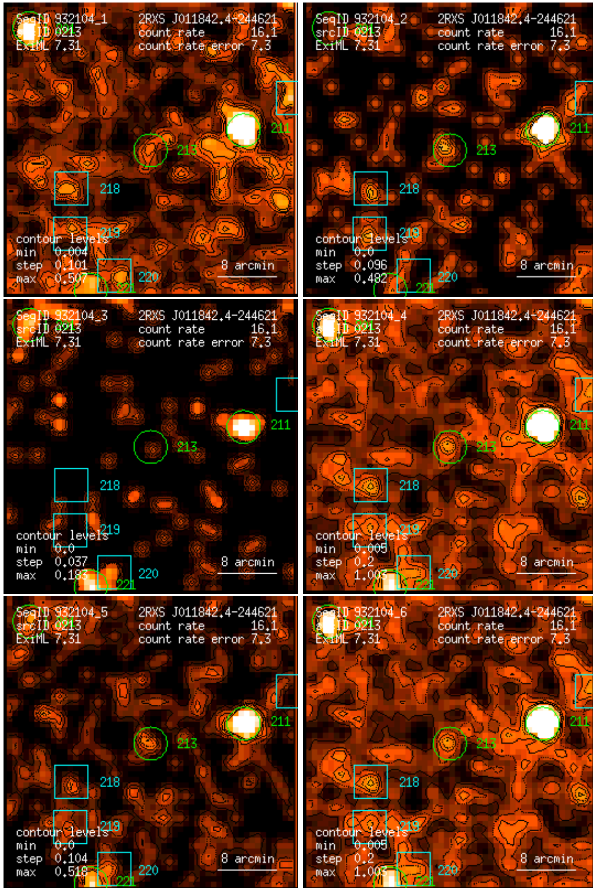
Figure 213: RASS 932104: detection 0213: band rate images, Gaussian filter: (1) PSPC channels 11 – 41, (2) 52 – 90, (3) 91 – 201, (4) 11 – 235, (5) 52 – 201, (6) 11 – 201. Broad band rates in counts/ks. Band rate contour levels in counts/ks/arcmin 2 .
