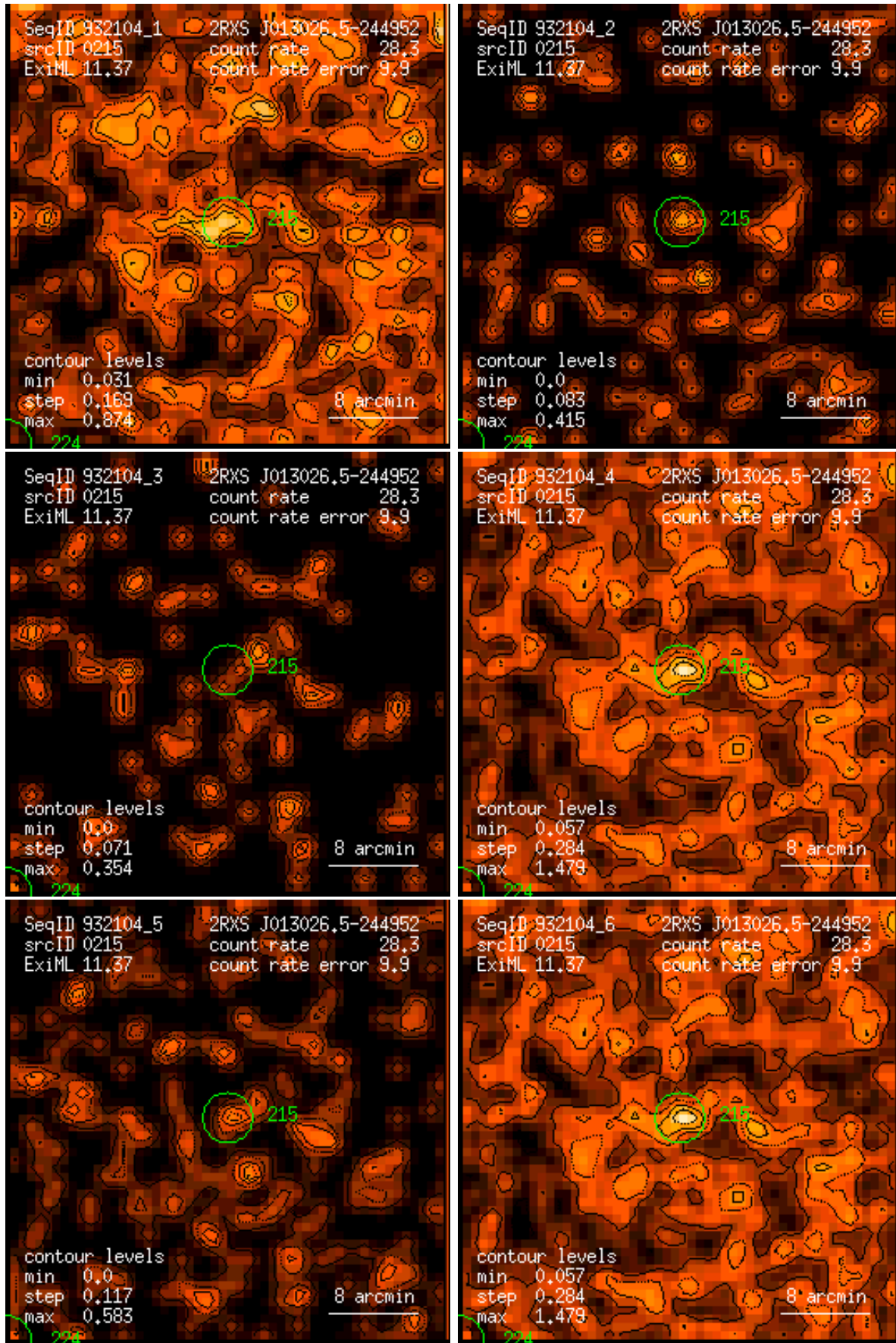
Figure 215: RASS 932104: detection 0215: band rate images, Gaussian filter: (1) PSPC channels 11 – 41, (2) 52 – 90, (3) 91 – 201, (4) 11 – 235, (5) 52 – 201, (6) 11 – 201. Broad band rates in counts/ks. Band rate contour levels in counts/ks/arcmin 2 .
