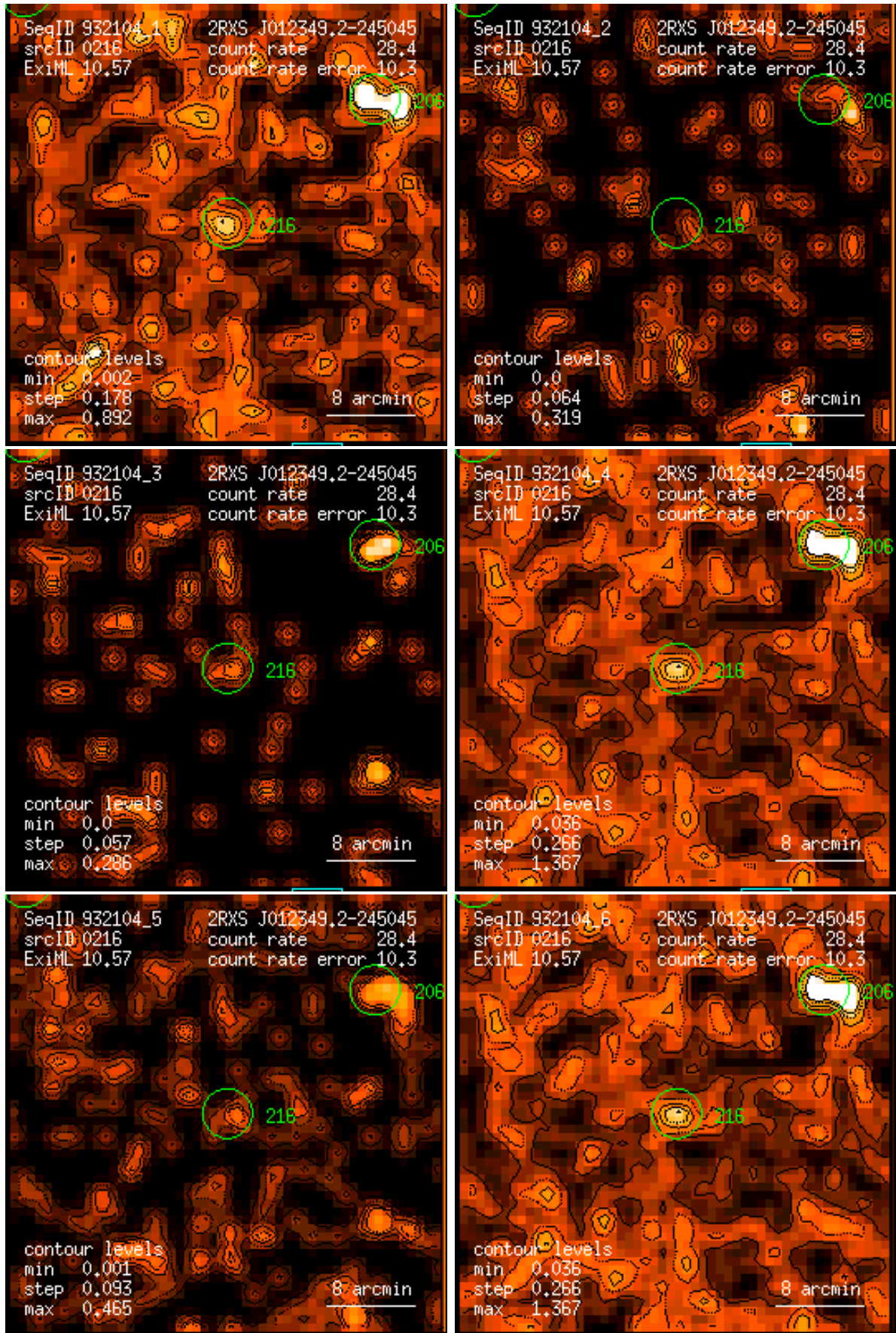
Figure 216: RASS 932104: detection 0216: band rate images, Gaussian filter: (1) PSPC channels 11 – 41, (2) 52 – 90, (3) 91 – 201, (4) 11 – 235, (5) 52 – 201, (6) 11 – 201. Broad band rates in counts/ks. Band rate contour levels in counts/ks/arcmin 2 .
