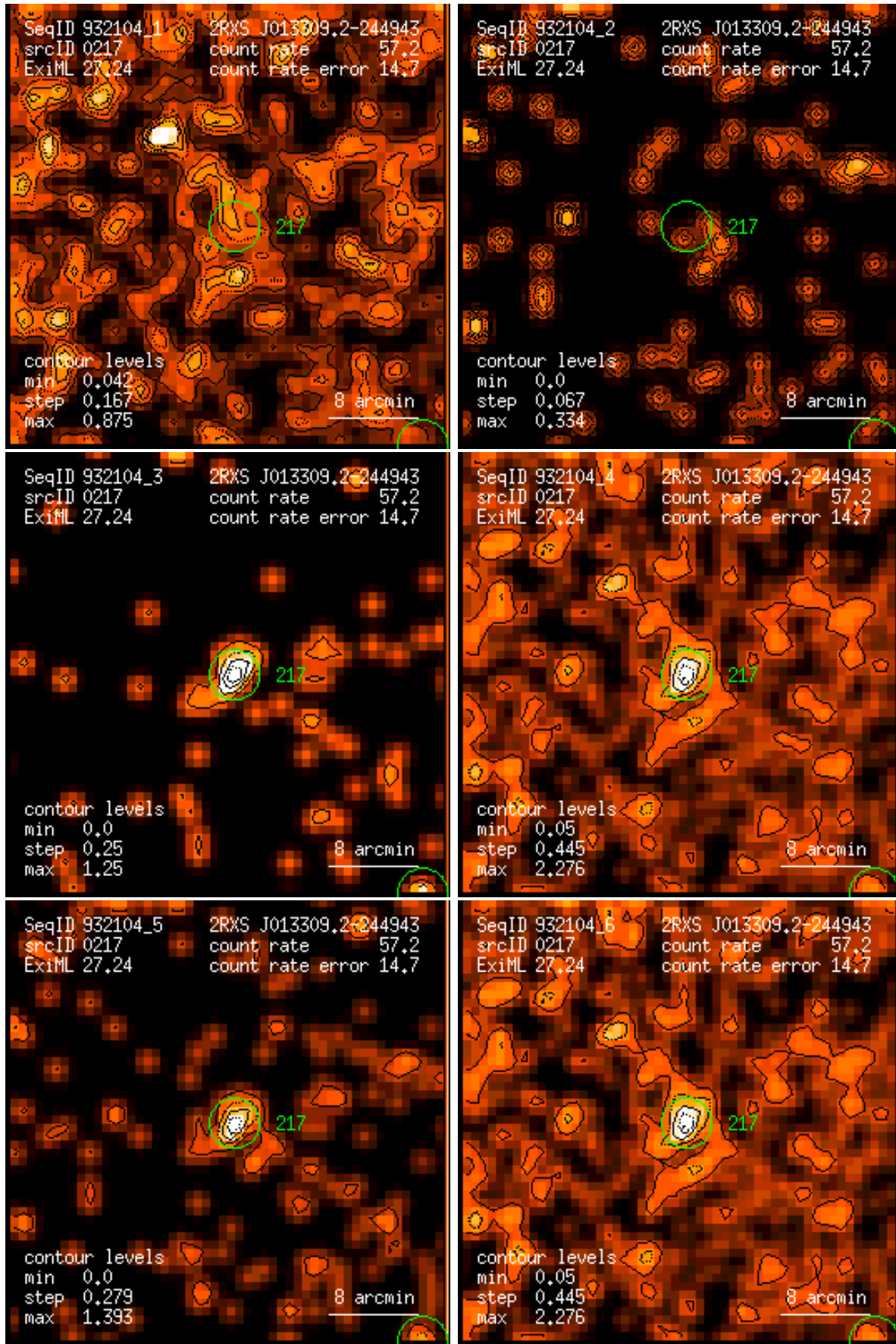
Figure 217: RASS 932104: detection 0217: band rate images, Gaussian filter: (1) PSPC channels 11 – 41, (2) 52 – 90, (3) 91 – 201, (4) 11 – 235, (5) 52 – 201, (6) 11 – 201. Broad band rates in counts/ks. Band rate contour levels in counts/ks/arcmin 2 .
