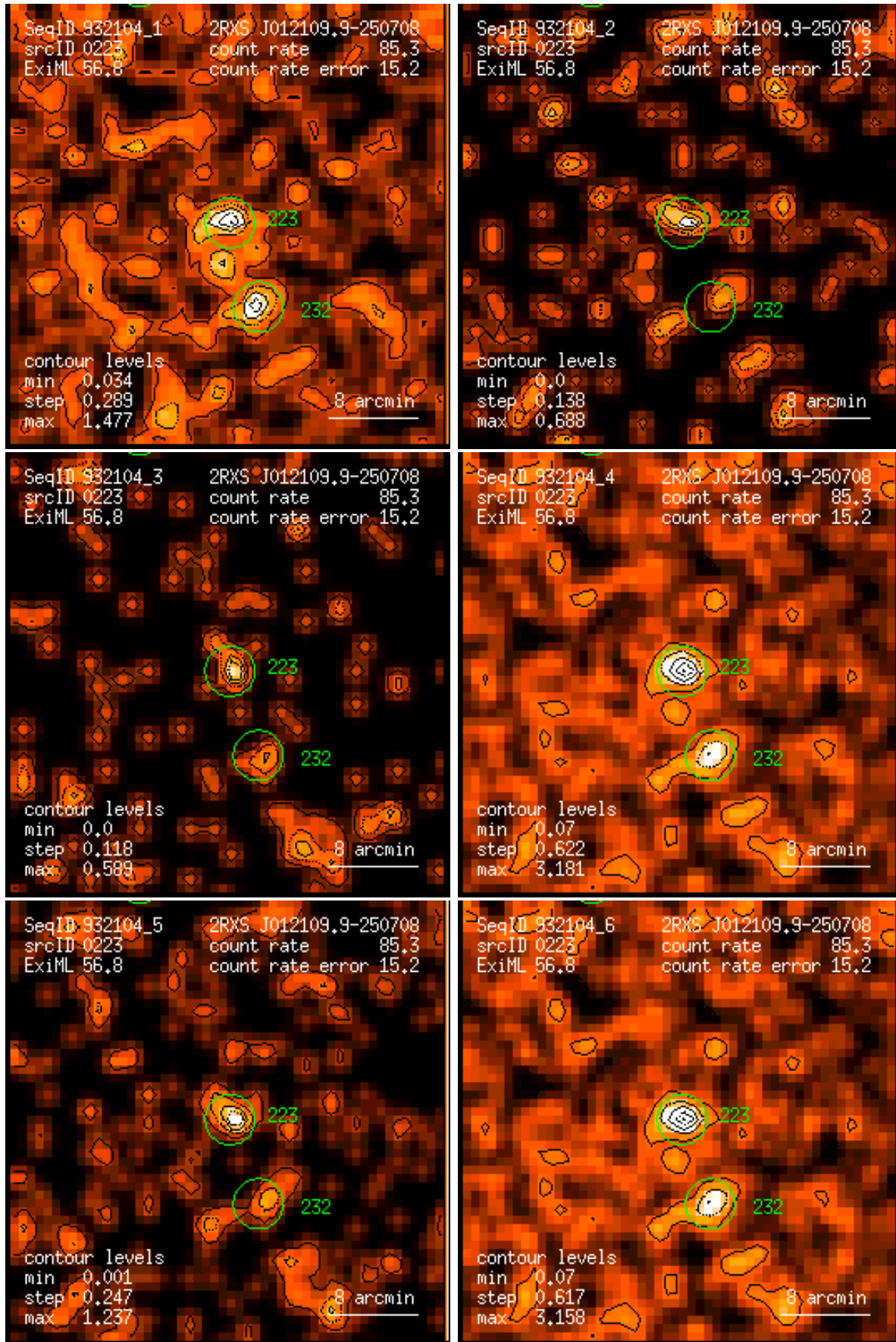
Figure 223: RASS 932104: detection 0223: band rate images, Gaussian filter: (1) PSPC channels 11 – 41, (2) 52 – 90, (3) 91 – 201, (4) 11 – 235, (5) 52 – 201, (6) 11 – 201. Broad band rates in counts/ks. Band rate contour levels in counts/ks/arcmin 2 .
