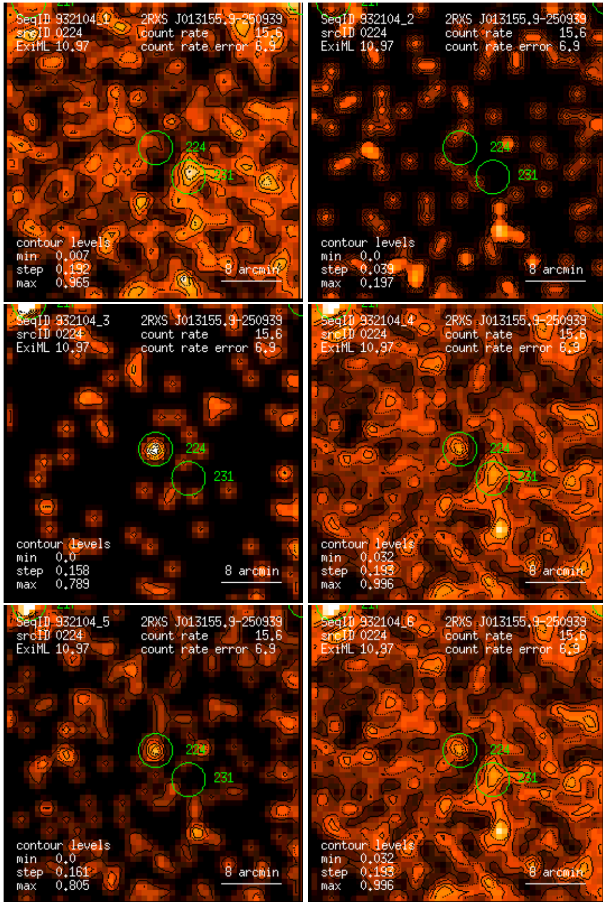
Figure 224: RASS 932104: detection 0224: band rate images, Gaussian filter: (1) PSPC channels 11 – 41, (2) 52 – 90, (3) 91 – 201, (4) 11 – 235, (5) 52 – 201, (6) 11 – 201. Broad band rates in counts/ks. Band rate contour levels in counts/ks/arcmin 2 .
