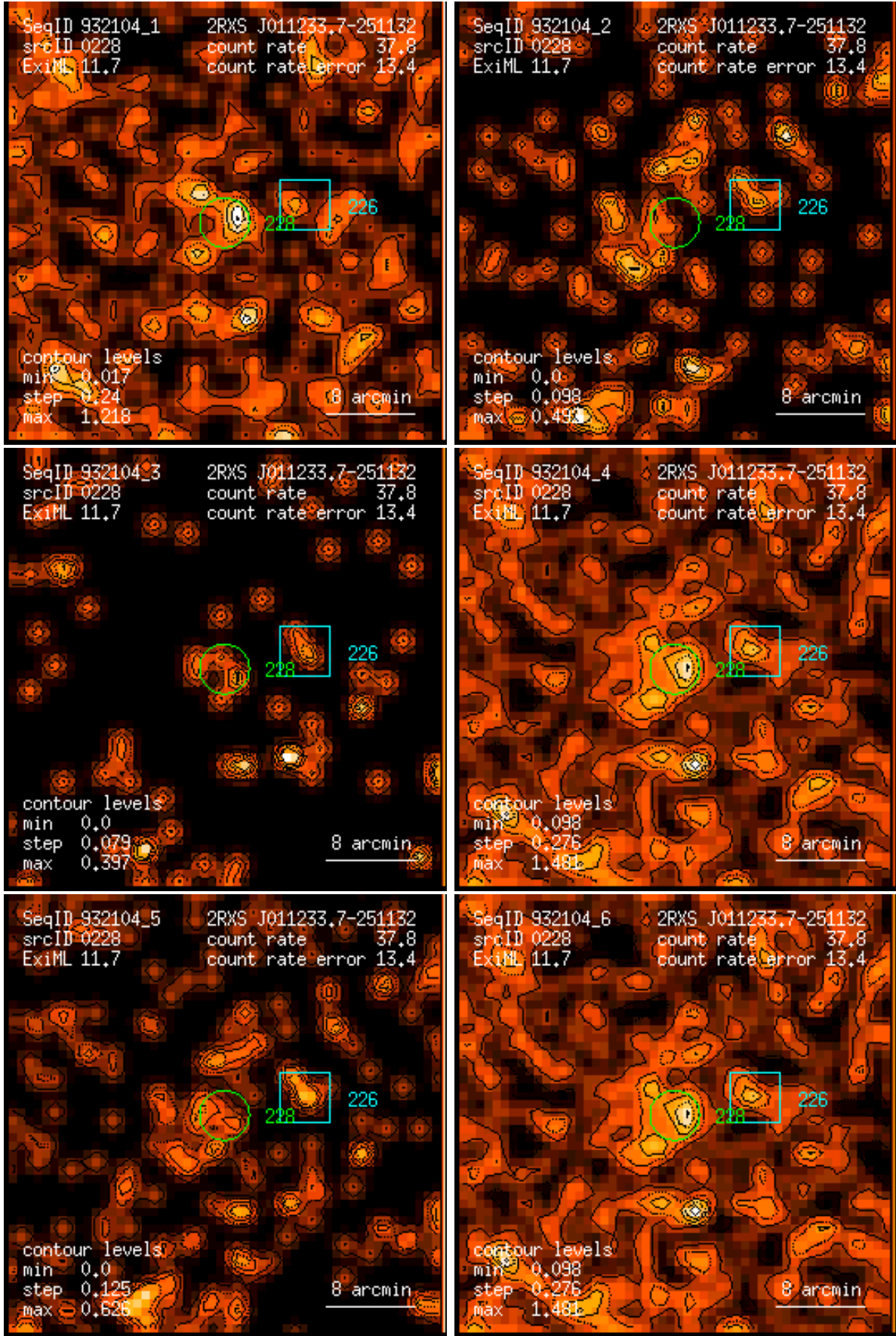
Figure 228: RASS 932104: detection 0228: band rate images, Gaussian filter: (1) PSPC channels 11 – 41, (2) 52 – 90, (3) 91 – 201, (4) 11 – 235, (5) 52 – 201, (6) 11 – 201. Broad band rates in counts/ks. Band rate contour levels in counts/ks/arcmin 2 .
