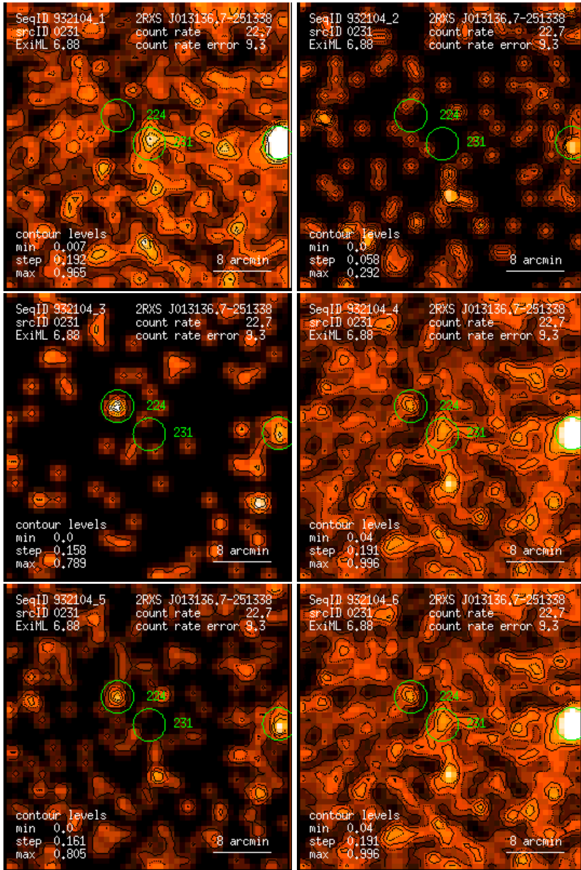
Figure 231: RASS 932104: detection 0231: band rate images, Gaussian filter: (1) PSPC channels 11 – 41, (2) 52 – 90, (3) 91 – 201, (4) 11 – 235, (5) 52 – 201, (6) 11 – 201. Broad band rates in counts/ks. Band rate contour levels in counts/ks/arcmin 2 .
