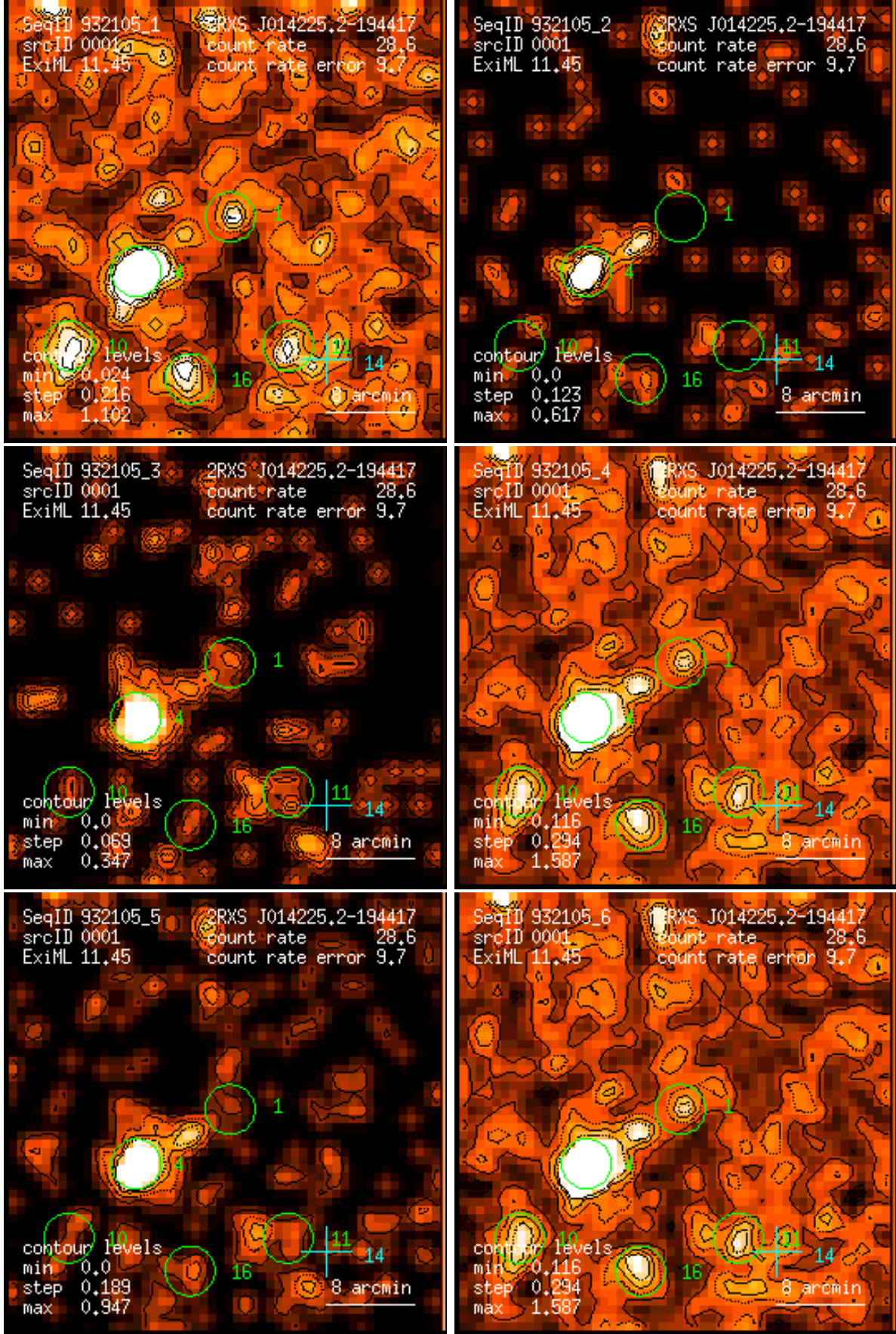
Figure 1: RASS 932105: detection 0001: band rate images, Gaussian filter: (1) PSPC channels 11 – 41, (2) 52 – 90, (3) 91 – 201, (4) 11 – 235, (5) 52 – 201, (6) 11 – 201. Broad band rates in counts/ks. Band rate contour levels in counts/ks/arcmin 2 .
