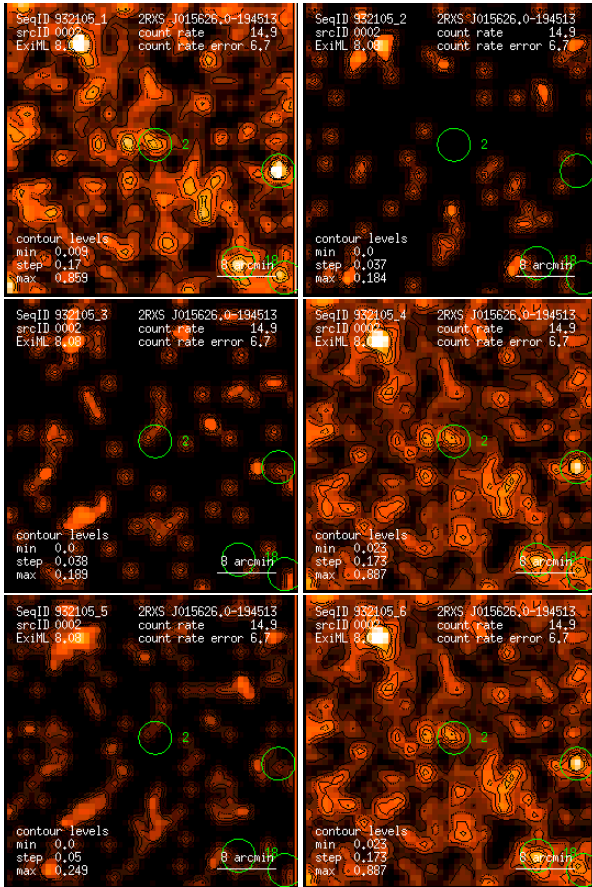
Figure 2: RASS 932105: detection 0002: band rate images, Gaussian filter: (1) PSPC channels 11 – 41, (2) 52 – 90, (3) 91 – 201, (4) 11 – 235, (5) 52 – 201, (6) 11 – 201. Broad band rates in counts/ks. Band rate contour levels in counts/ks/arcmin 2 .
