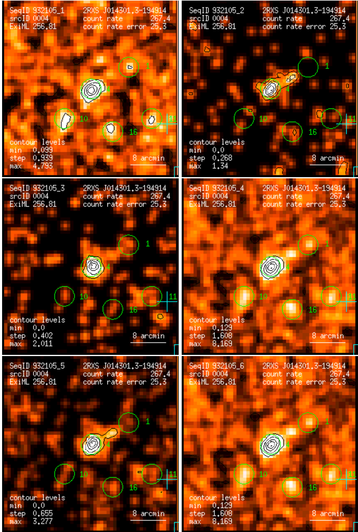
Figure 4: RASS 932105: detection 0004: band rate images, Gaussian filter: (1) PSPC channels 11 – 41, (2) 52 – 90, (3) 91 – 201, (4) 11 – 235, (5) 52 – 201, (6) 11 – 201. Broad band rates in counts/ks. Band rate contour levels in counts/ks/arcmin 2 .
