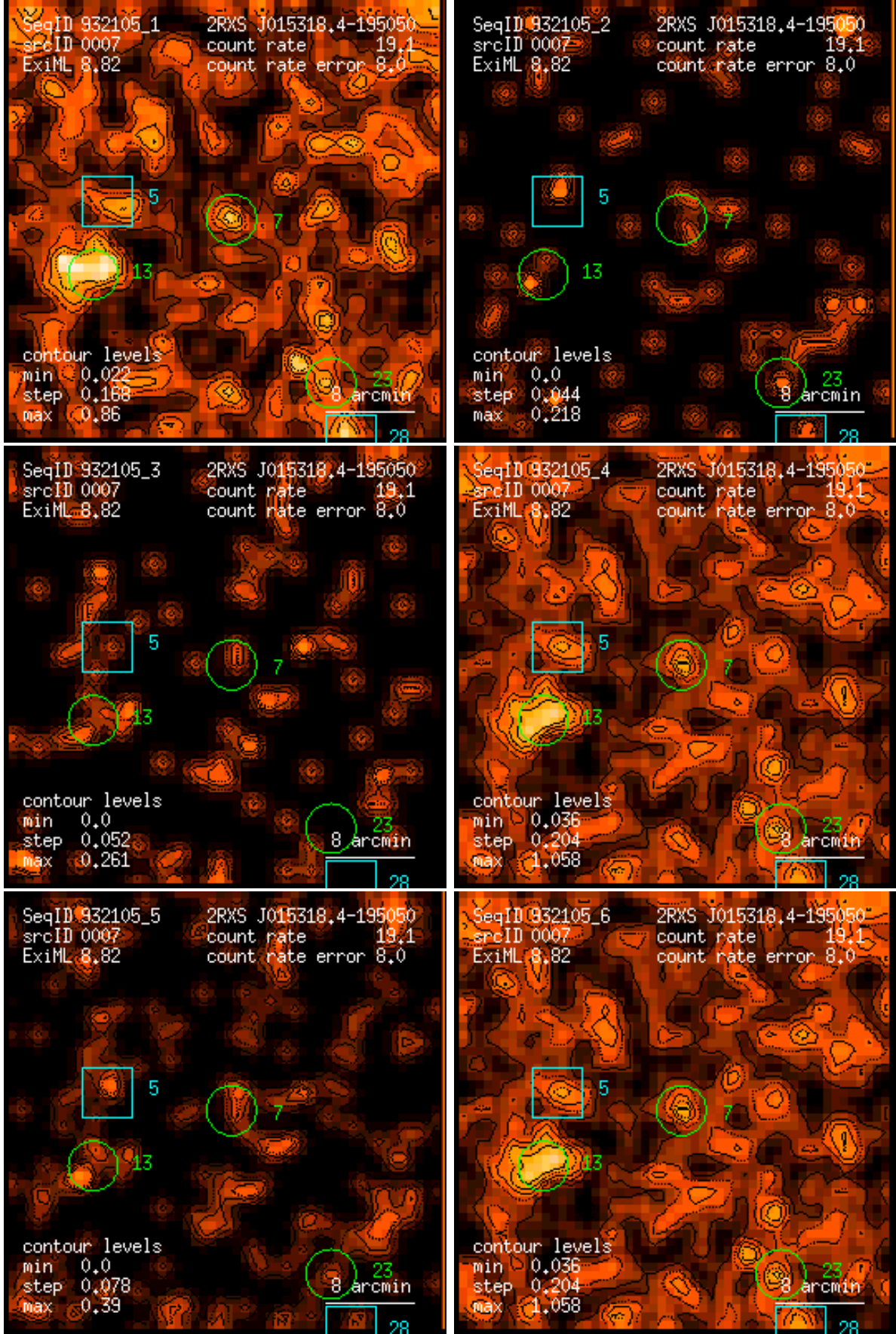
Figure 7: RASS 932105: detection 0007: band rate images, Gaussian filter: (1) PSPC channels 11 – 41, (2) 52 – 90, (3) 91 – 201, (4) 11 – 235, (5) 52 – 201, (6) 11 – 201. Broad band rates in counts/ks. Band rate contour levels in counts/ks/arcmin 2 .
