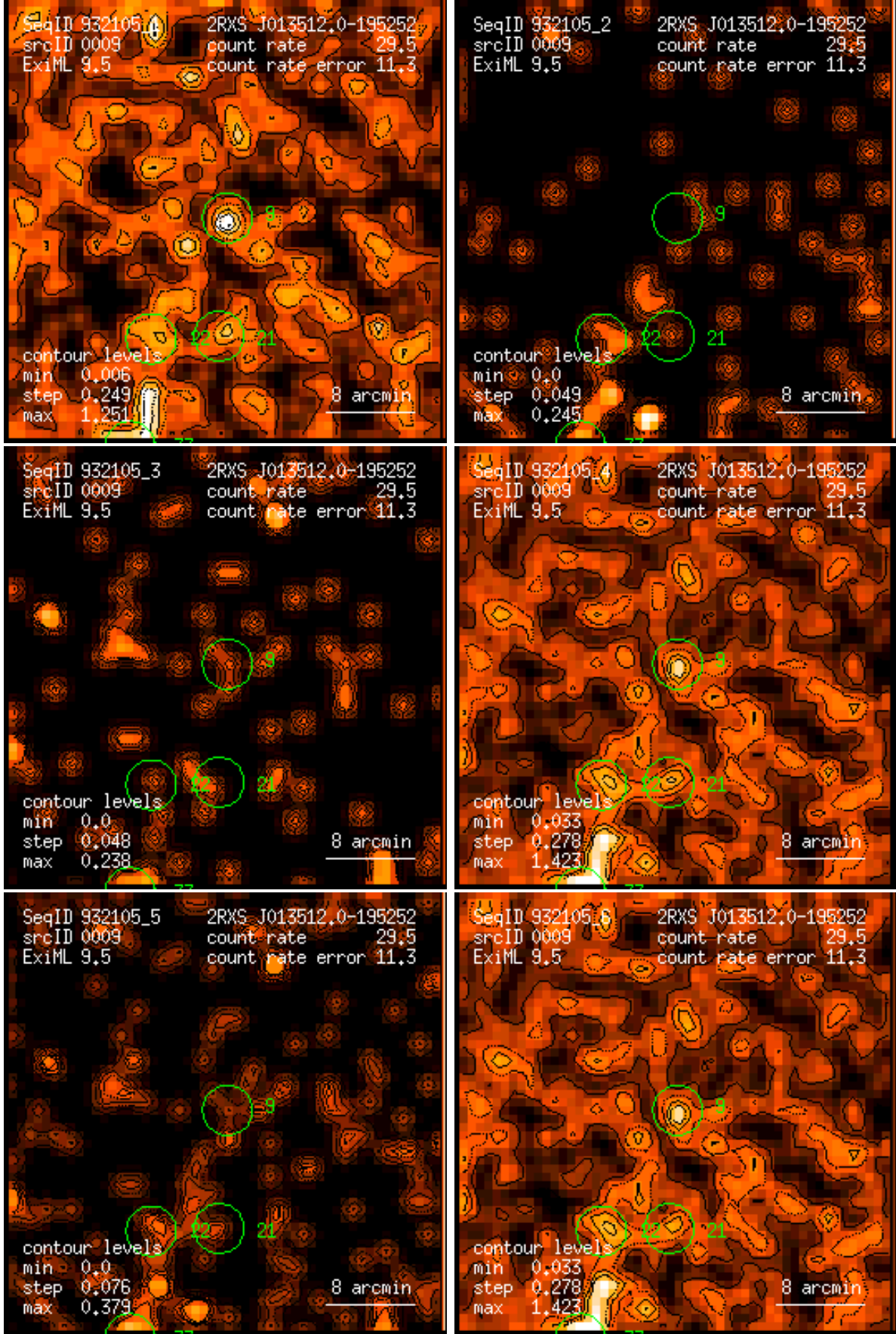
Figure 9: RASS 932105: detection 0009: band rate images, Gaussian filter: (1) PSPC channels 11 – 41, (2) 52 – 90, (3) 91 – 201, (4) 11 – 235, (5) 52 – 201, (6) 11 – 201. Broad band rates in counts/ks. Band rate contour levels in counts/ks/arcmin 2 .
