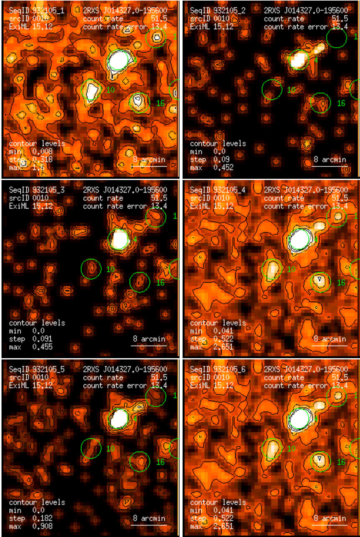
Figure 10: RASS 932105: detection 0010: band rate images, Gaussian filter: (1) PSPC channels 11 – 41, (2) 52 – 90, (3) 91 – 201, (4) 11 – 235, (5) 52 – 201, (6) 11 – 201. Broad band rates in counts/ks. Band rate contour levels in counts/ks/arcmin 2 .
