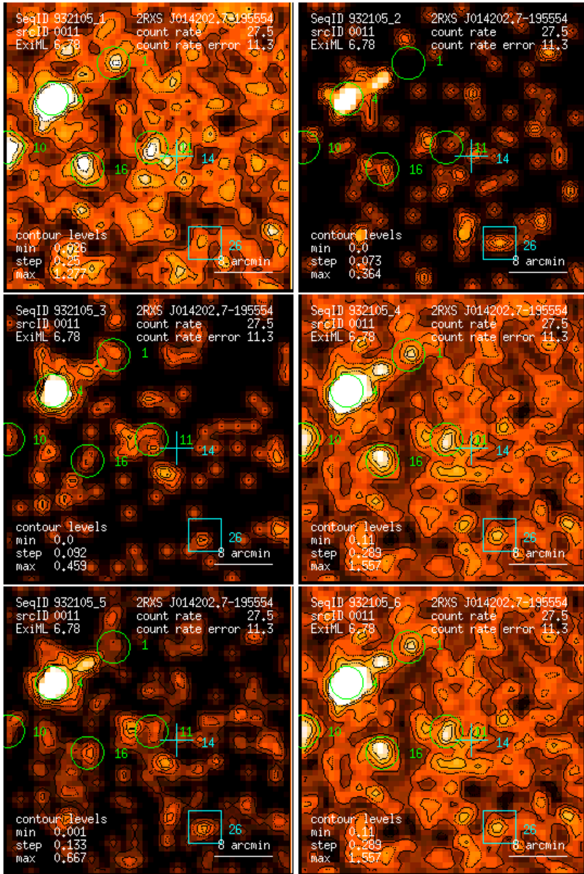
Figure 11: RASS 932105: detection 0011: band rate images, Gaussian filter: (1) PSPC channels 11 – 41, (2) 52 – 90, (3) 91 – 201, (4) 11 – 235, (5) 52 – 201, (6) 11 – 201. Broad band rates in counts/ks. Band rate contour levels in counts/ks/arcmin 2 .
