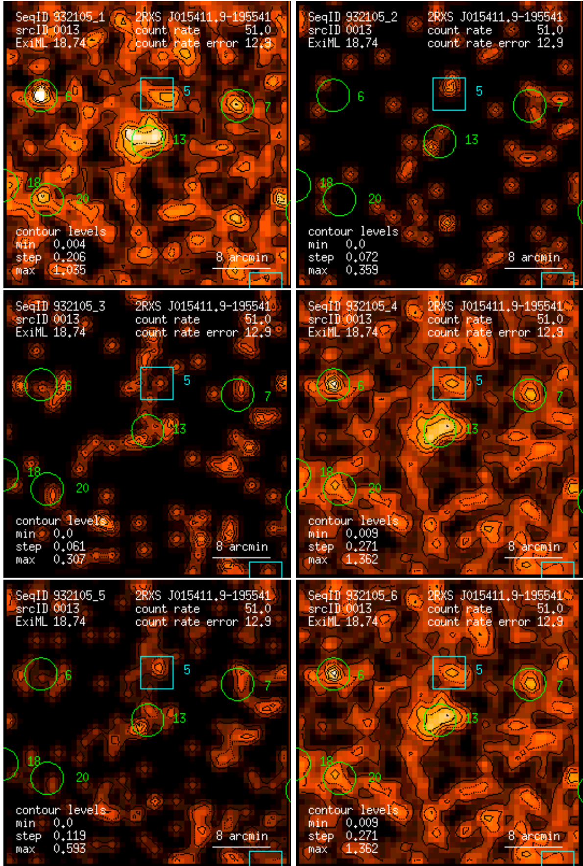
Figure 13: RASS 932105: detection 0013: band rate images, Gaussian filter: (1) PSPC channels 11 – 41, (2) 52 – 90, (3) 91 – 201, (4) 11 – 235, (5) 52 – 201, (6) 11 – 201. Broad band rates in counts/ks. Band rate contour levels in counts/ks/arcmin 2 .
