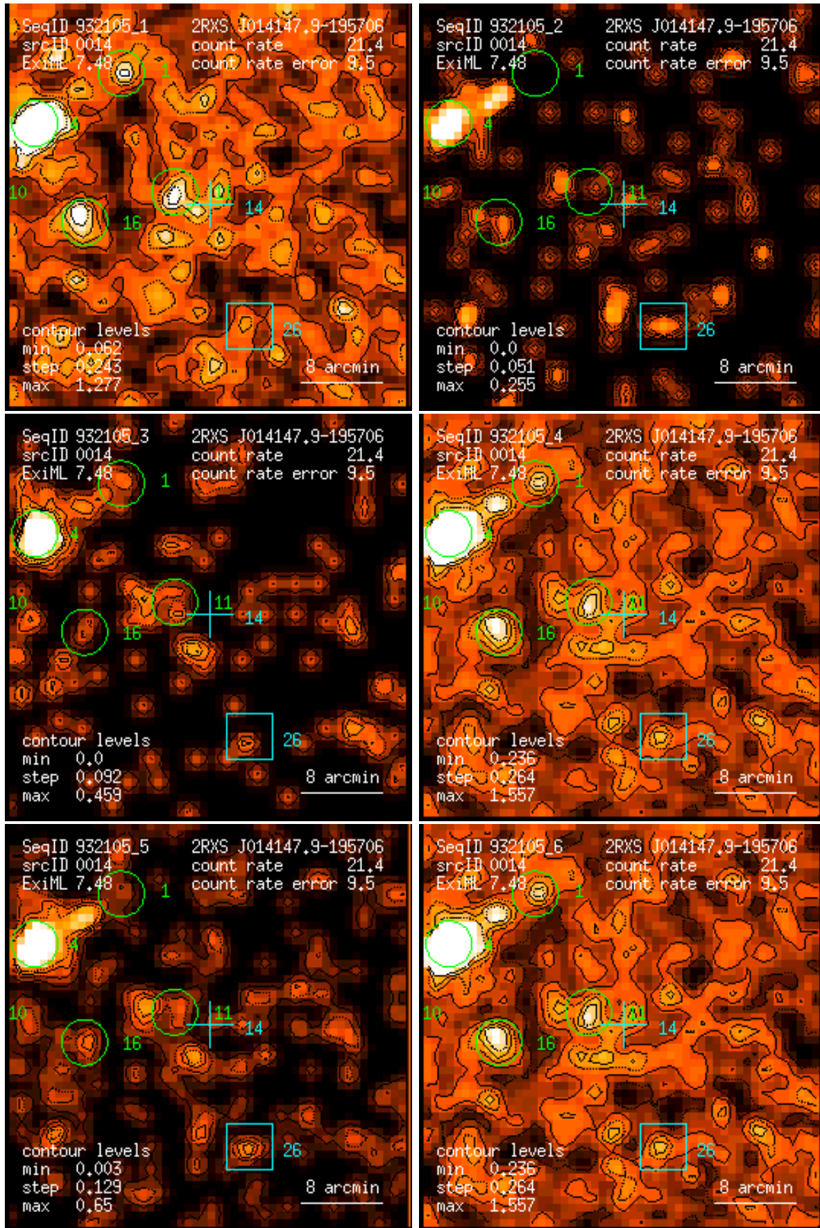
Figure 14: RASS 932105: detection 0014: band rate images, Gaussian filter: (1) PSPC channels 11 – 41, (2) 52 – 90, (3) 91 – 201, (4) 11 – 235, (5) 52 – 201, (6) 11 – 201. Broad band rates in counts/ks. Band rate contour levels in counts/ks/arcmin 2 .
