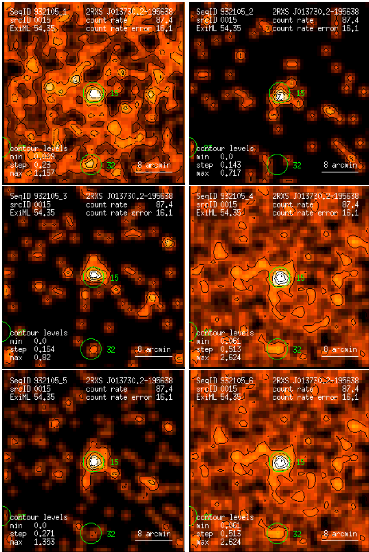
Figure 15: RASS 932105: detection 0015: band rate images, Gaussian filter: (1) PSPC channels 11 – 41, (2) 52 – 90, (3) 91 – 201, (4) 11 – 235, (5) 52 – 201, (6) 11 – 201. Broad band rates in counts/ks. Band rate contour levels in counts/ks/arcmin 2 .
