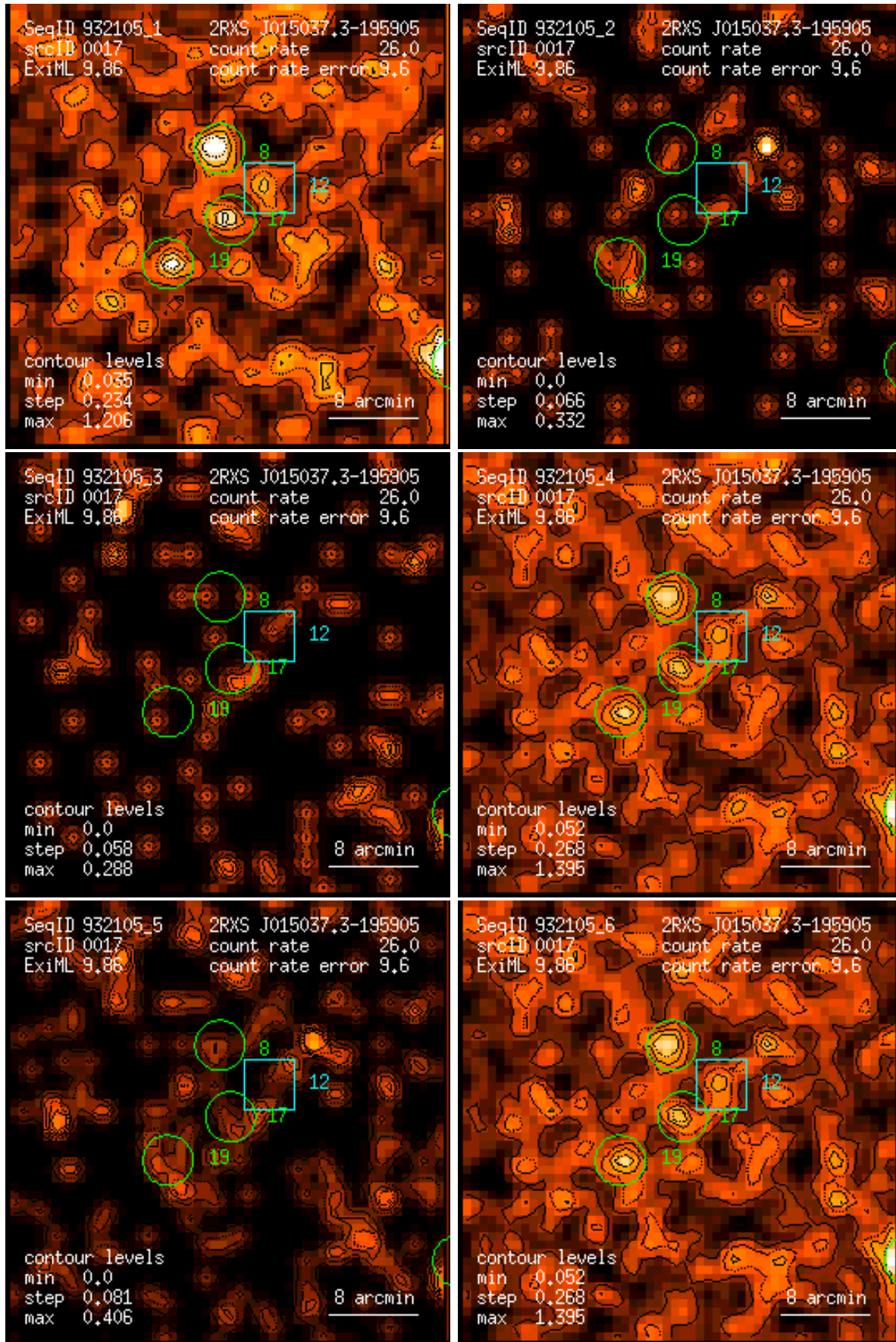
Figure 17: RASS 932105: detection 0017: band rate images, Gaussian filter: (1) PSPC channels 11 – 41, (2) 52 – 90, (3) 91 – 201, (4) 11 – 235, (5) 52 – 201, (6) 11 – 201. Broad band rates in counts/ks. Band rate contour levels in counts/ks/arcmin 2 .
