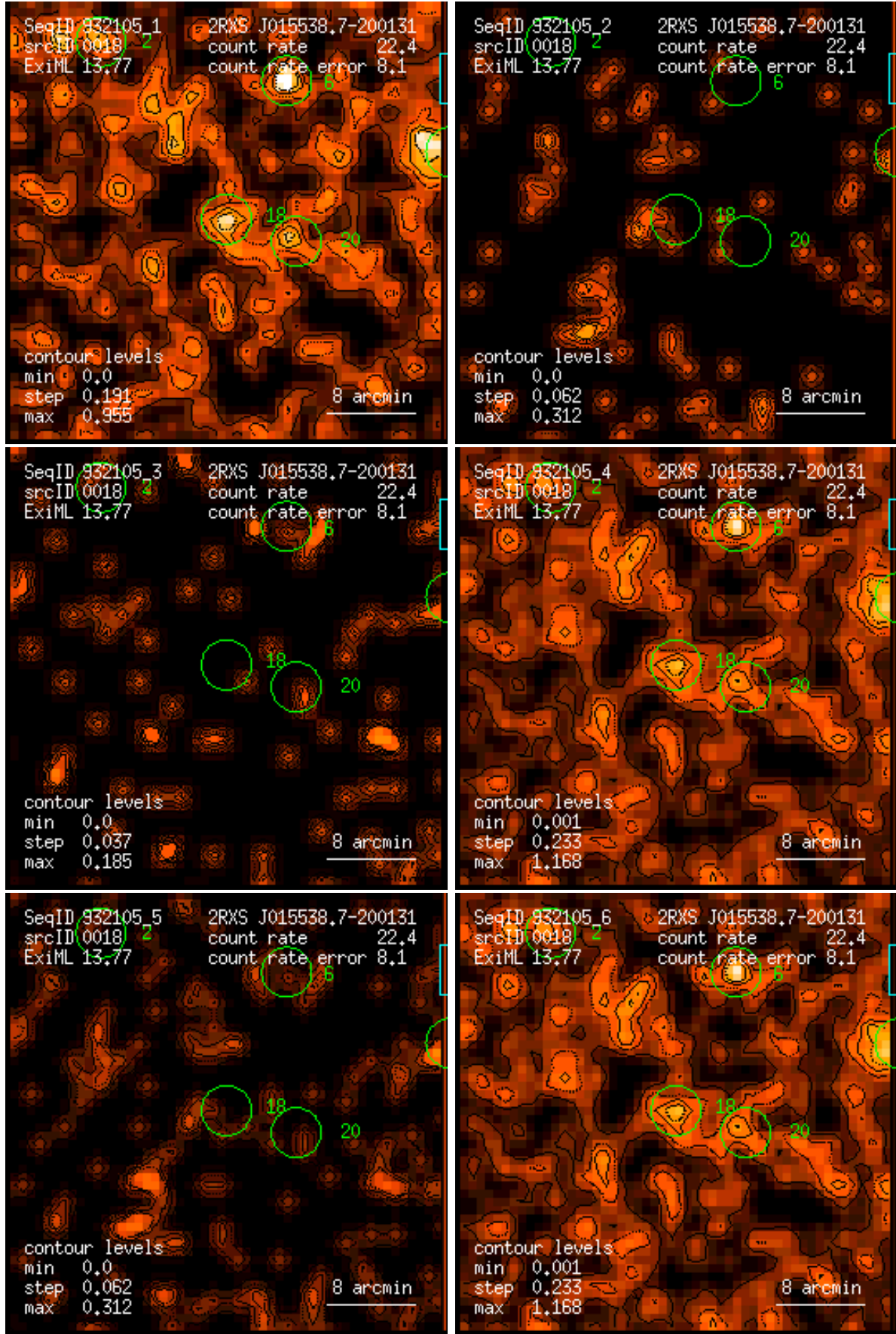
Figure 18: RASS 932105: detection 0018: band rate images, Gaussian filter: (1) PSPC channels 11 – 41, (2) 52 – 90, (3) 91 – 201, (4) 11 – 235, (5) 52 – 201, (6) 11 – 201. Broad band rates in counts/ks. Band rate contour levels in counts/ks/arcmin 2 .
