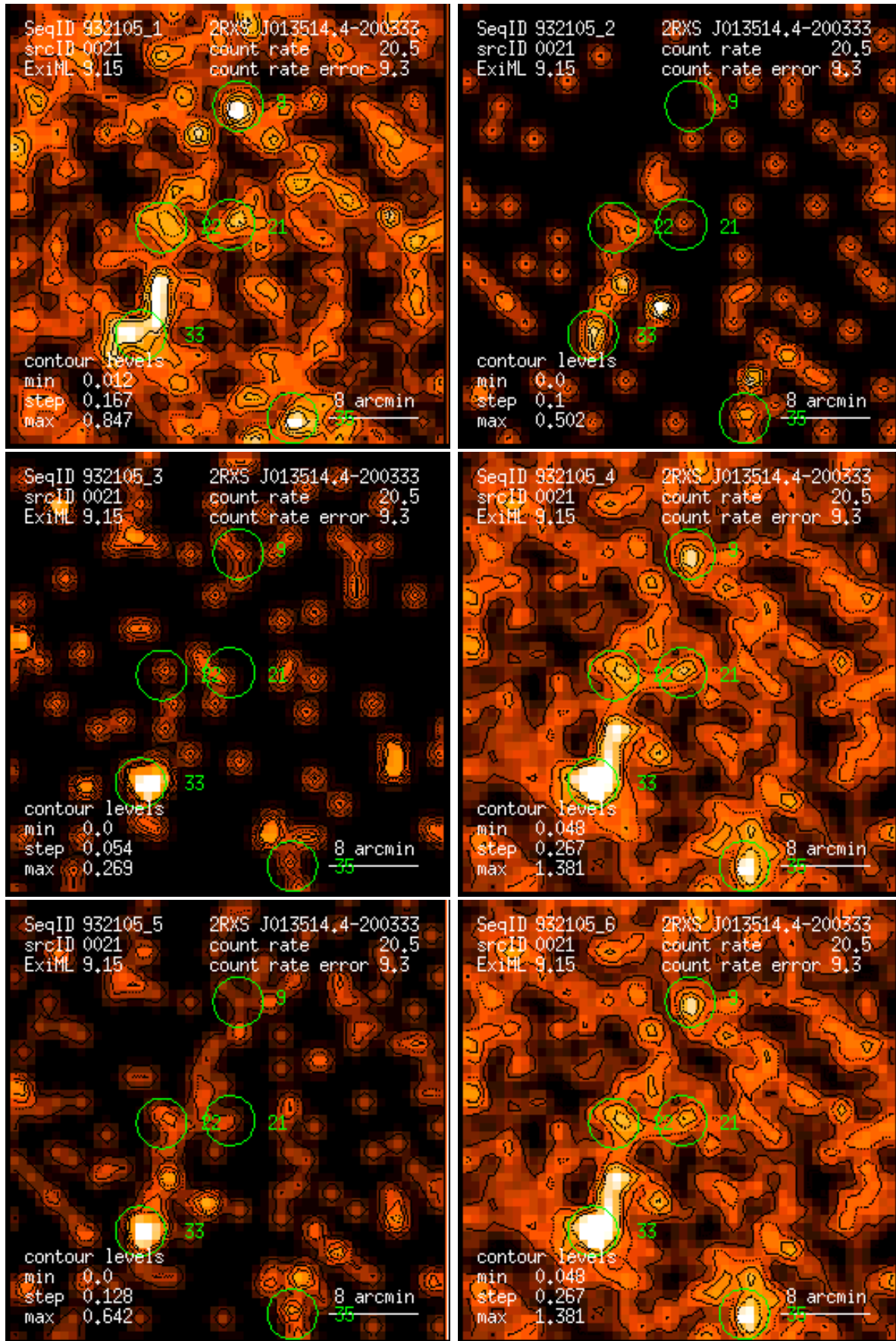
Figure 21: RASS 932105: detection 0021: band rate images, Gaussian filter: (1) PSPC channels 11 – 41, (2) 52 – 90, (3) 91 – 201, (4) 11 – 235, (5) 52 – 201, (6) 11 – 201. Broad band rates in counts/ks. Band rate contour levels in counts/ks/arcmin 2 .
